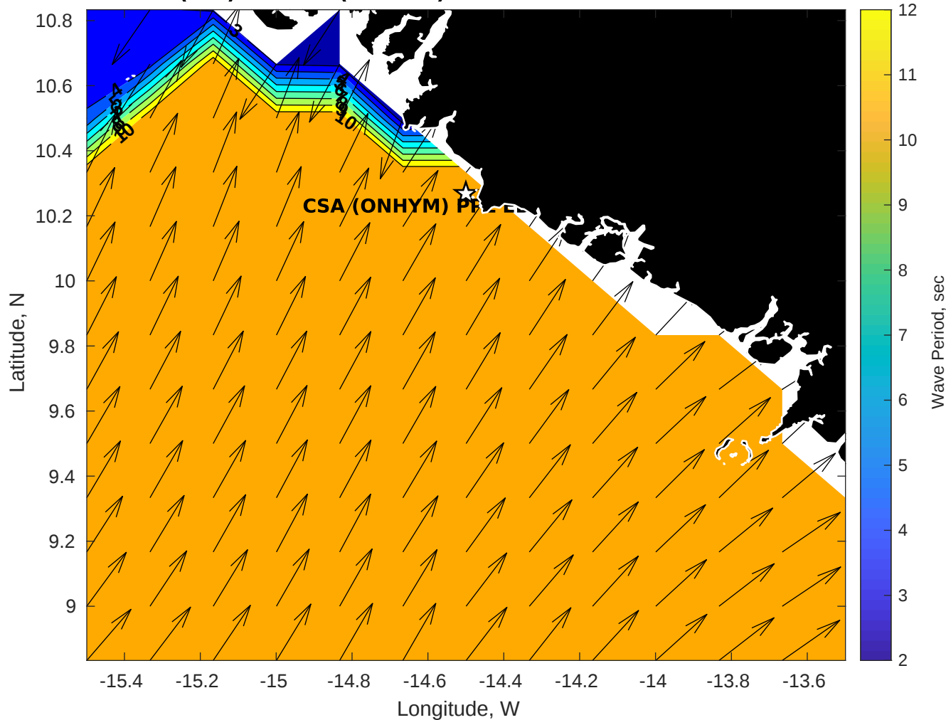
GFS Wave Period (sec) for CSA (ONHYM) PPL EBS - Guinea at 19-Dec-2025 09:00:00
