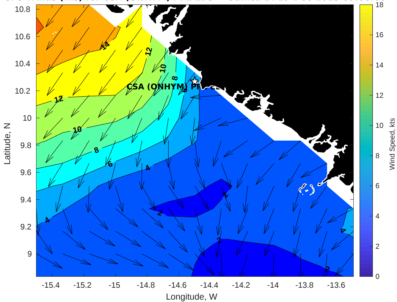
GFS Winds (kts) for CSA (ONHYM) PPL EBS - Guinea at 19-Dec-2025 09:00:00
