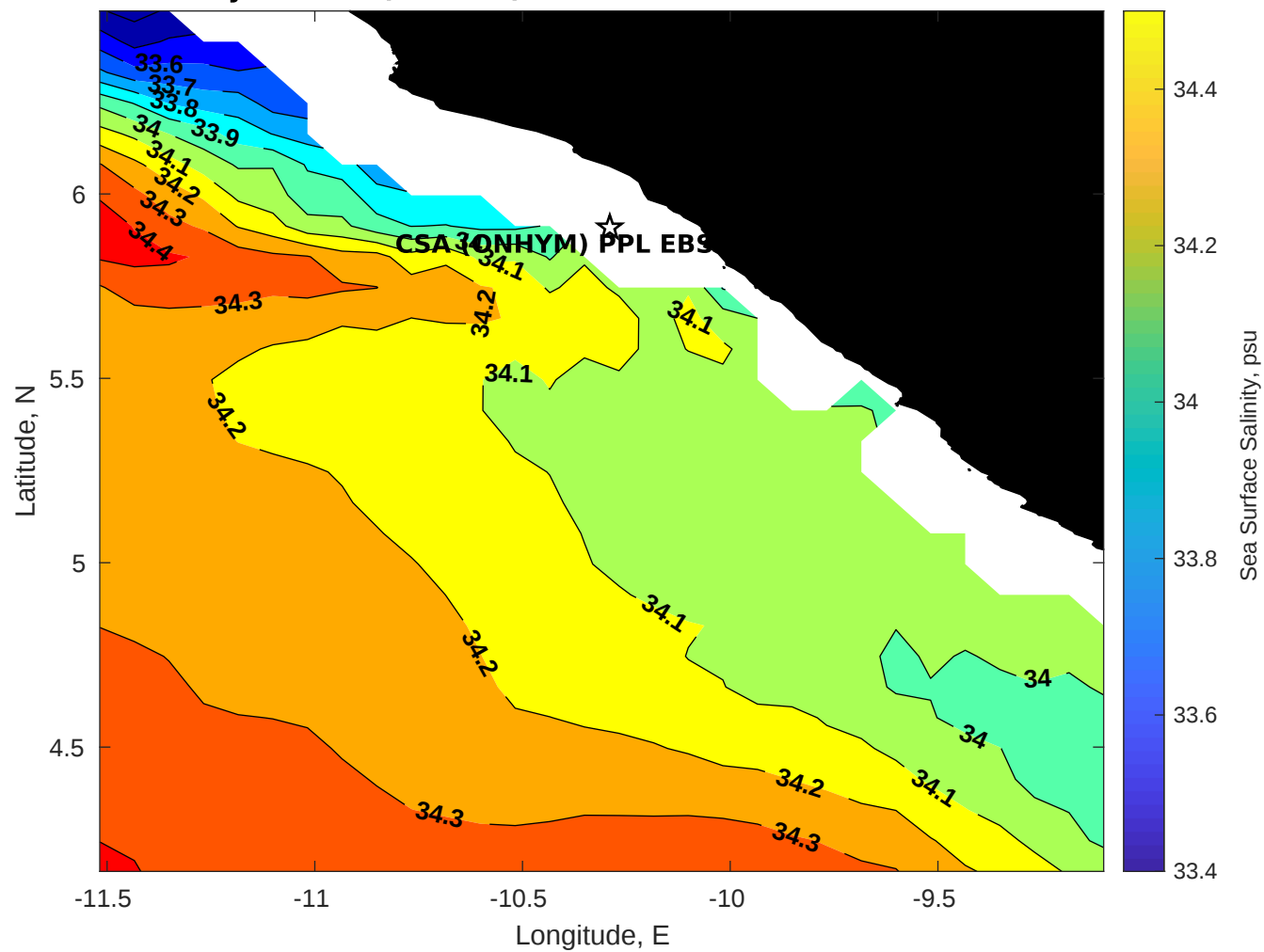
Surface Salinity for CSA (ONHYM) PPL EBS - Liberia at 18-Dec-2025 00:00:00
