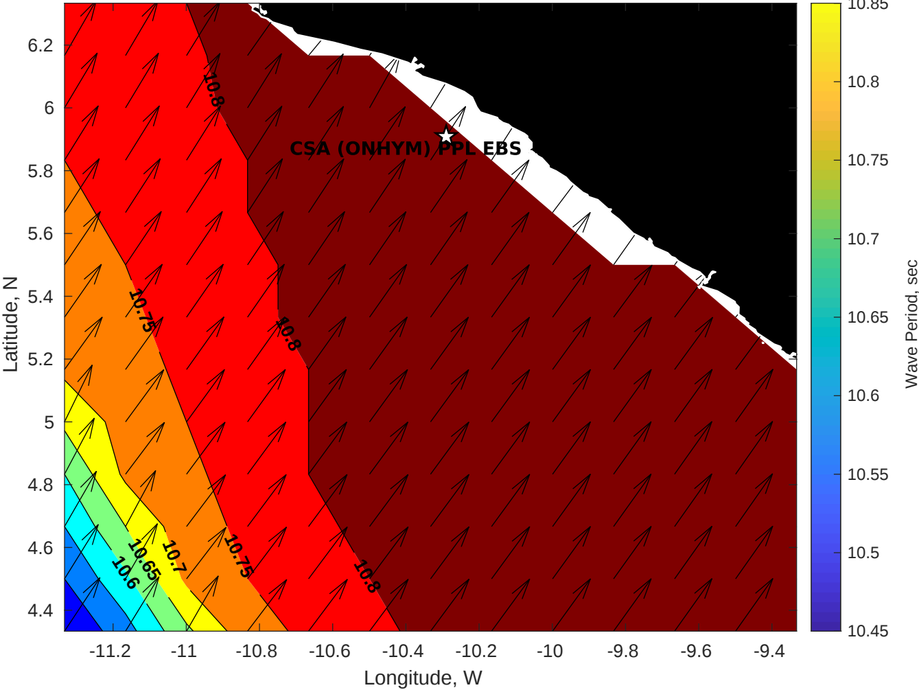
GFS Wave Period (sec) for CSA (ONHYM) PPL EBS - Liberia at 19-Dec-2025 09:00:00
