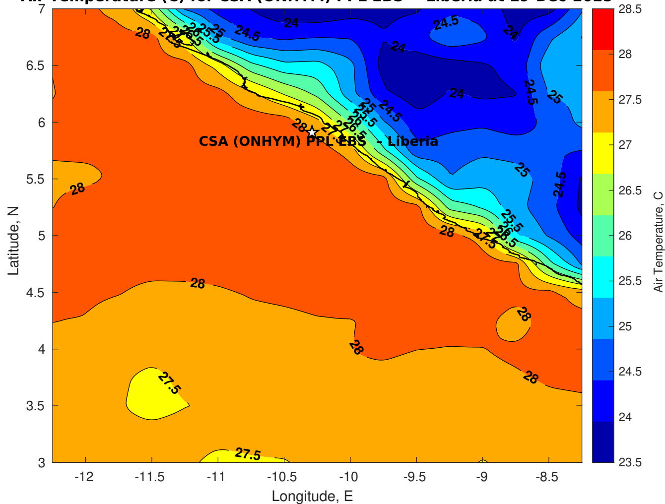
Air Temperature (C) for CSA (ONHYM) PPL EBS - Liberia at 19-Dec-2025
