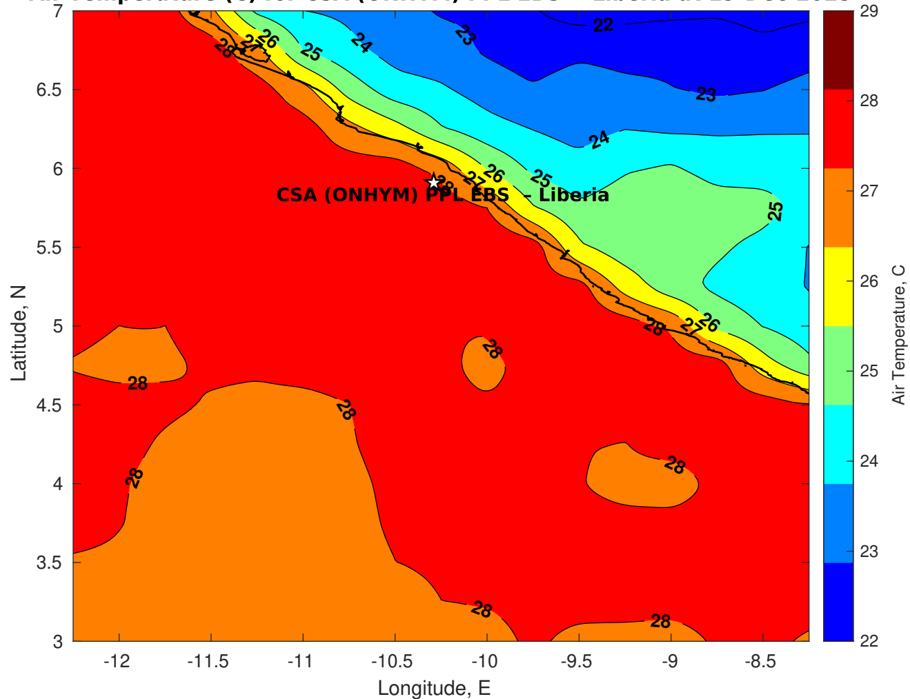
Air Temperature (C) for CSA (ONHYM) PPL EBS - Liberia at 19-Dec-2025
