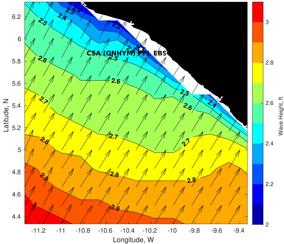
GFS Wave Height (ft) for CSA (ONHYM) PPL EBS - Liberia at 19-Dec-2025 09:00:00
