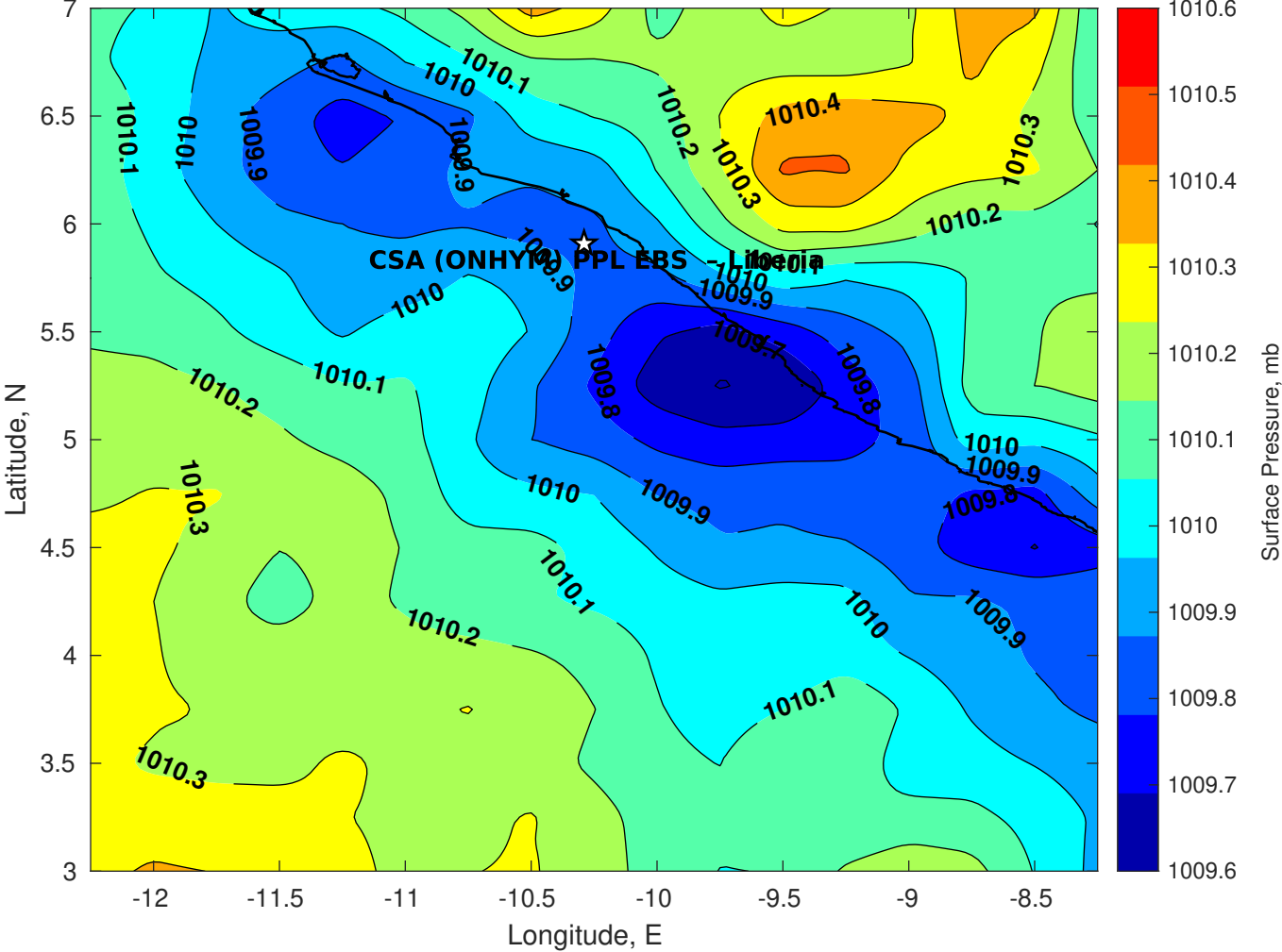
Surface Pressure (mb) for CSA (ONHYM) PPL EBS - Liberia at 21-Dec-2025 00:00:00
