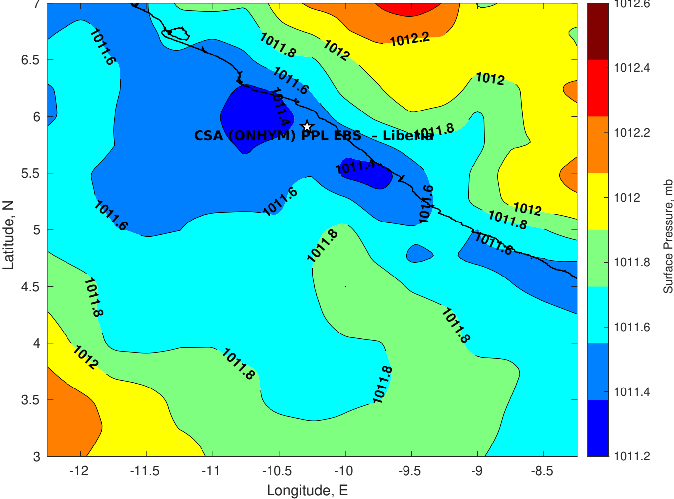
Surface Pressure (mb) for CSA (ONHYM) PPL EBS - Liberia at 19-Dec-2025 00:00:00
