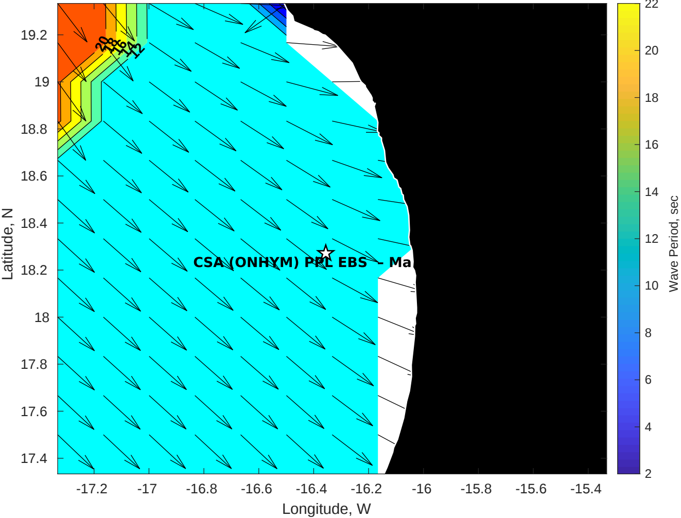
GFS Wave Period (sec) for CSA (ONHYM) PPL EBS - Mauritania at 19-Dec-2025 09:00:00
