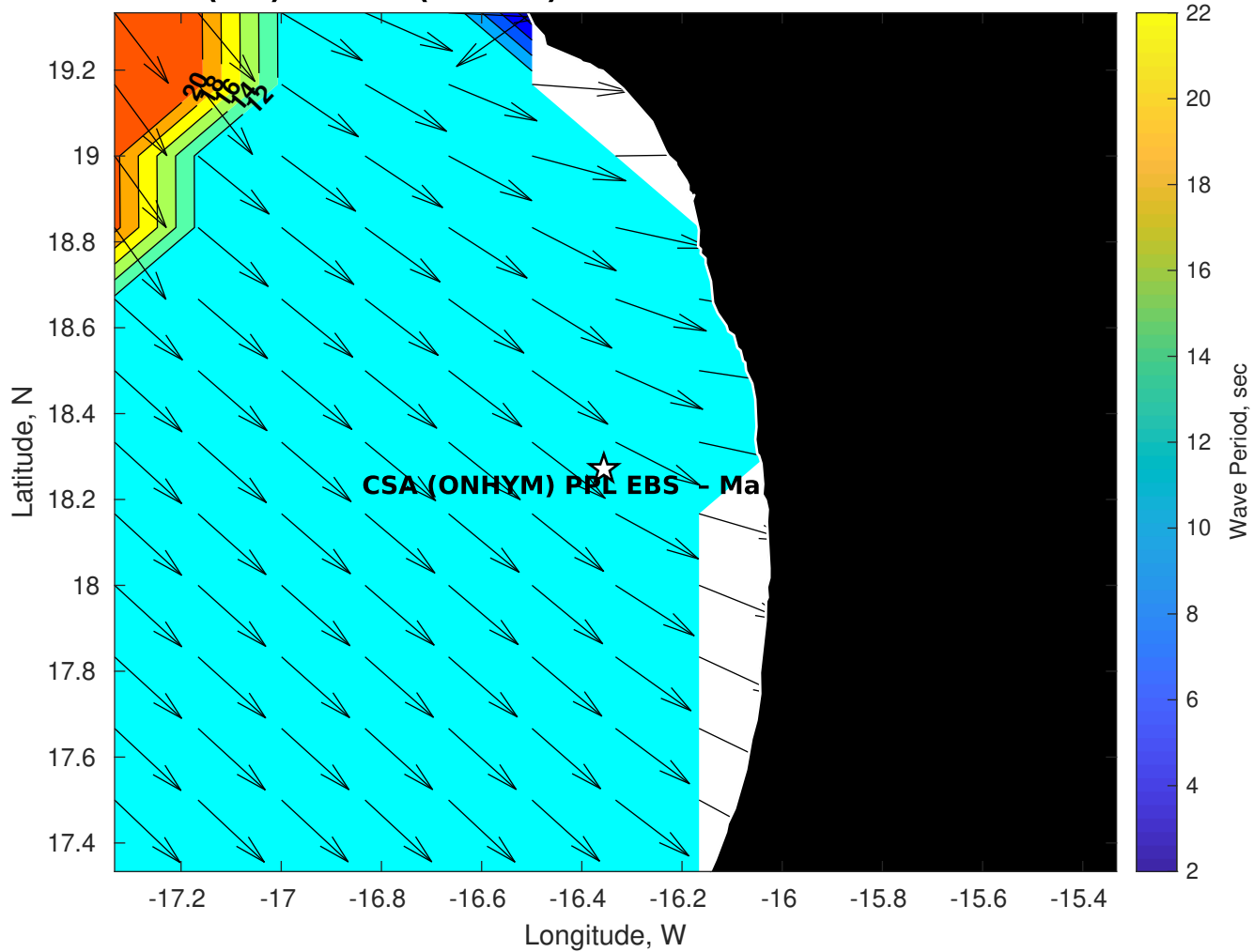
GFS Wave Period (sec) for CSA (ONHYM) PPL EBS - Mauritania at 19-Dec-2025 09:00:00
