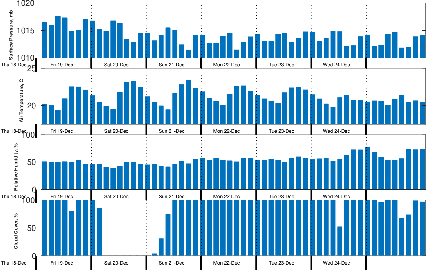
Met Forecast for CSA (ONHYM) PPL EBS - Mauritania from 19-Dec-2025 00:00:00 to 26-Dec-2025 00:00:00
