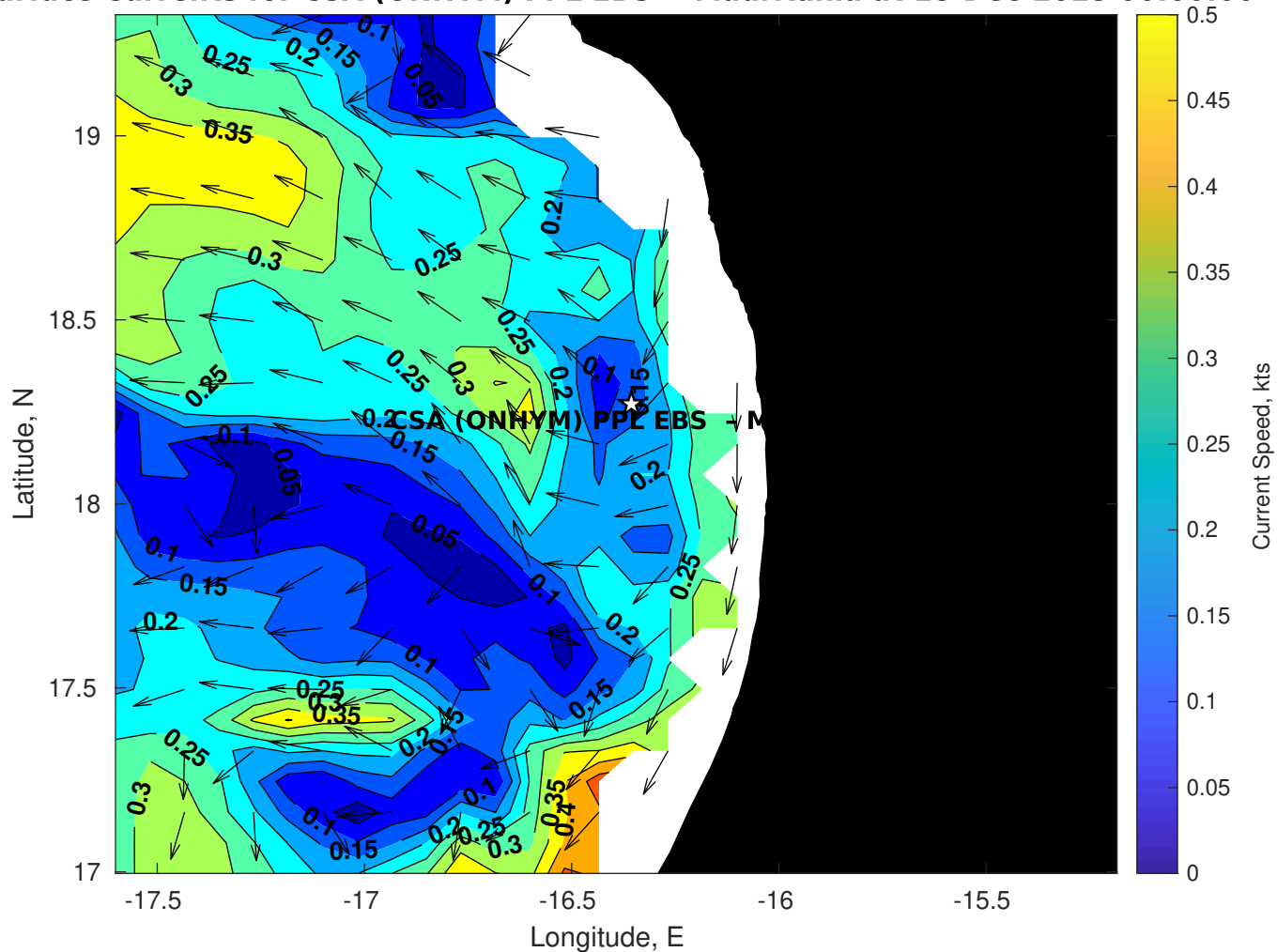
Surface Currents for CSA (ONHYM) PPL EBS - Mauritania at 18-Dec-2025 00:00:00
