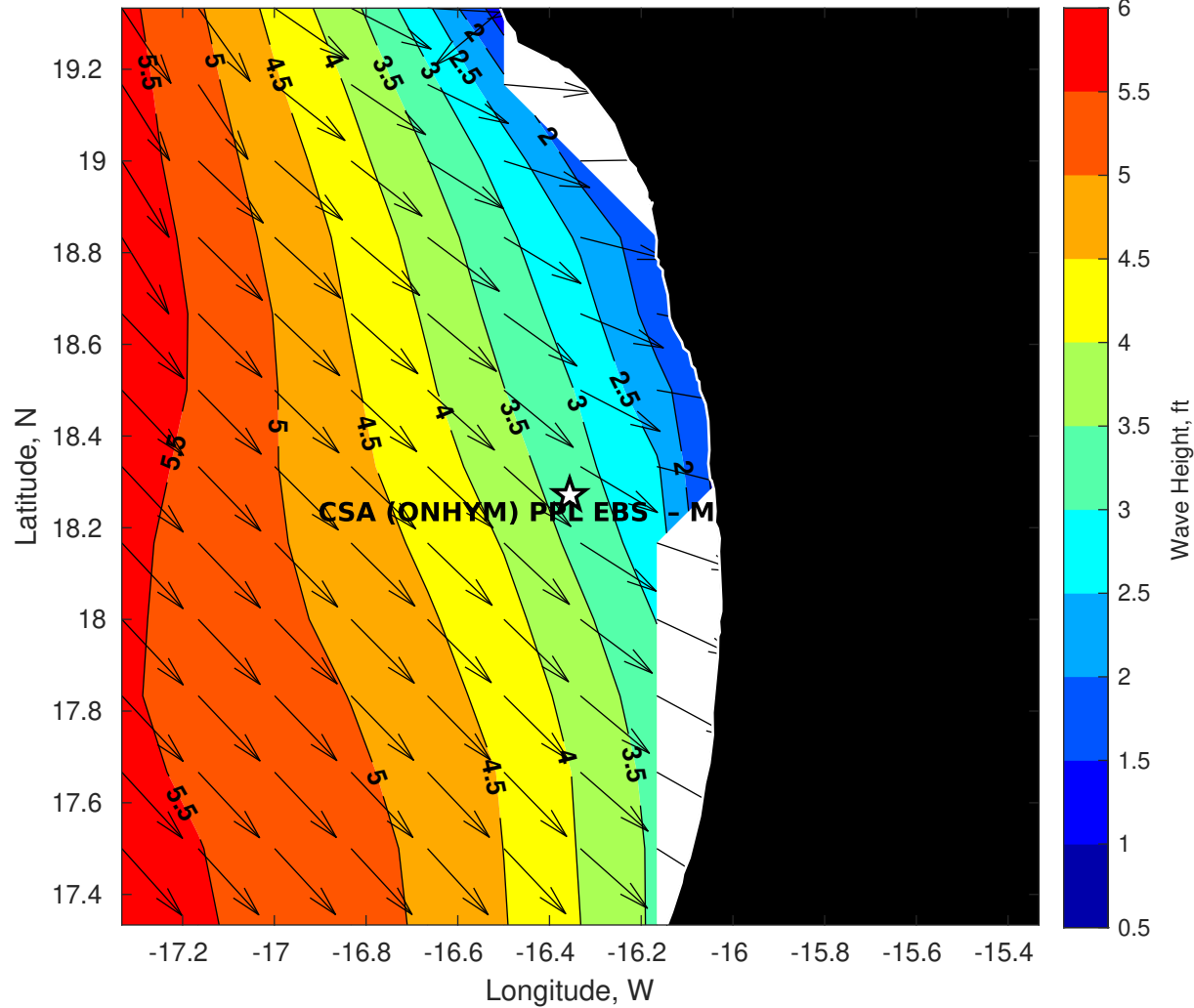
GFS Wave Height (ft) for CSA (ONHYM) PPL EBS - Mauritania at 19-Dec-2025 09:00:00
