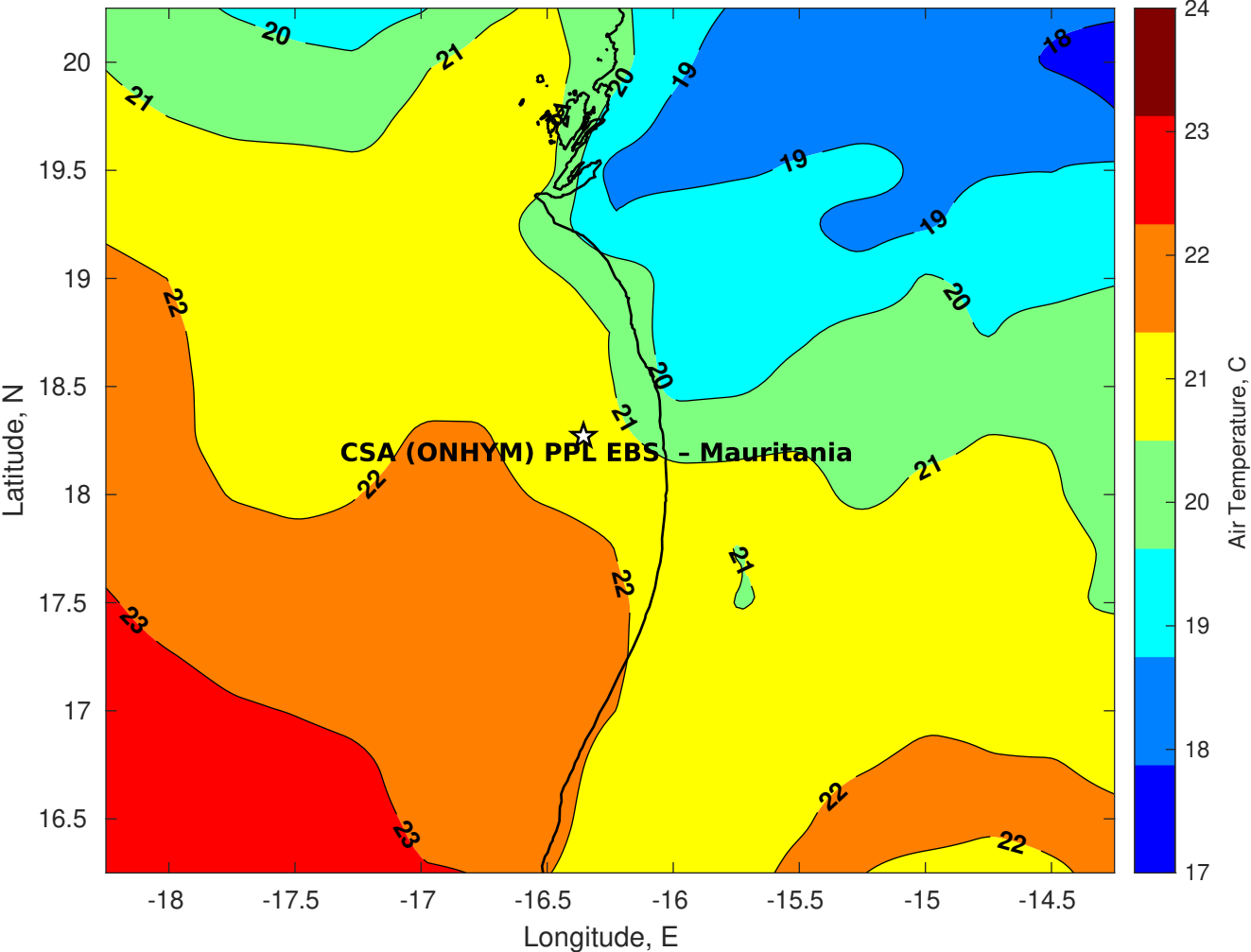
Air Temperature (C) for CSA (ONHYM) PPL EBS - Mauritania at 19-Dec-2025
