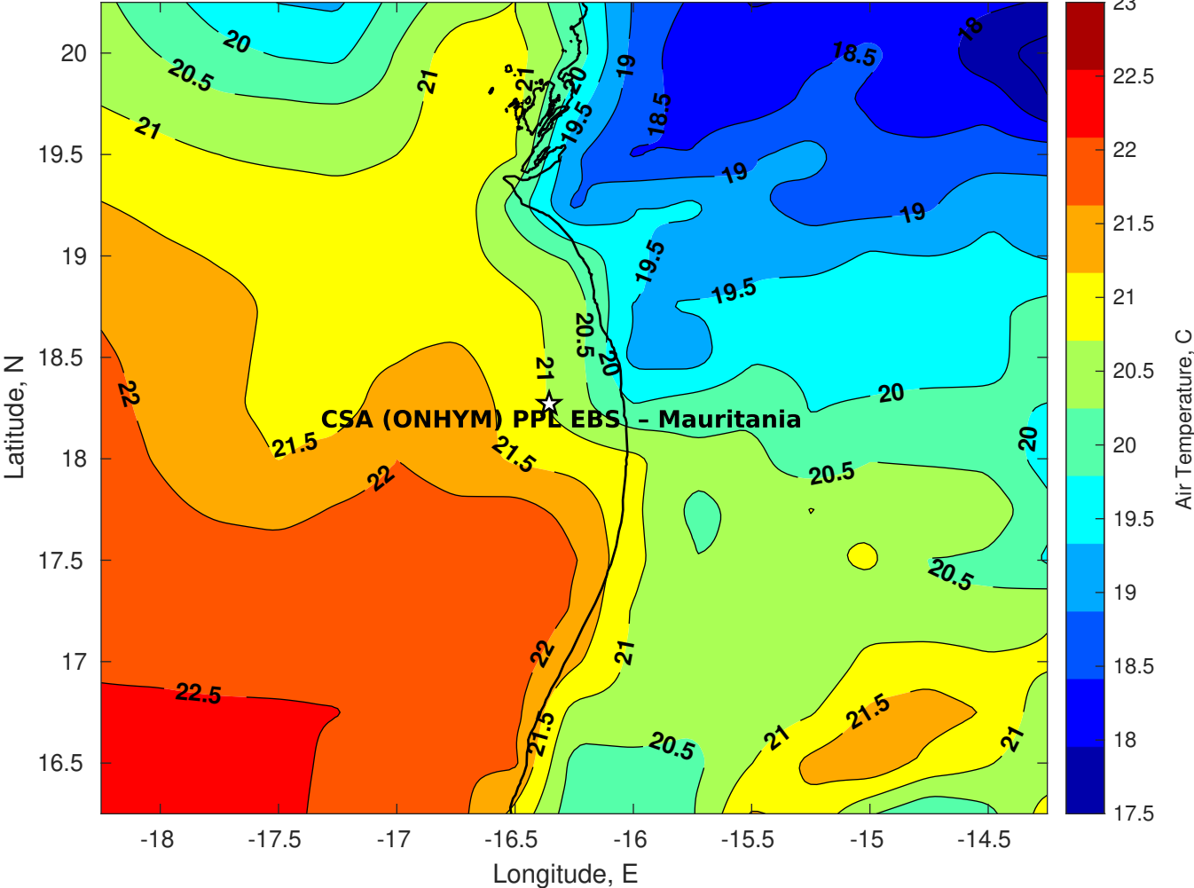
Air Temperature (C) for CSA (ONHYM) PPL EBS - Mauritania at 19-Dec-2025
