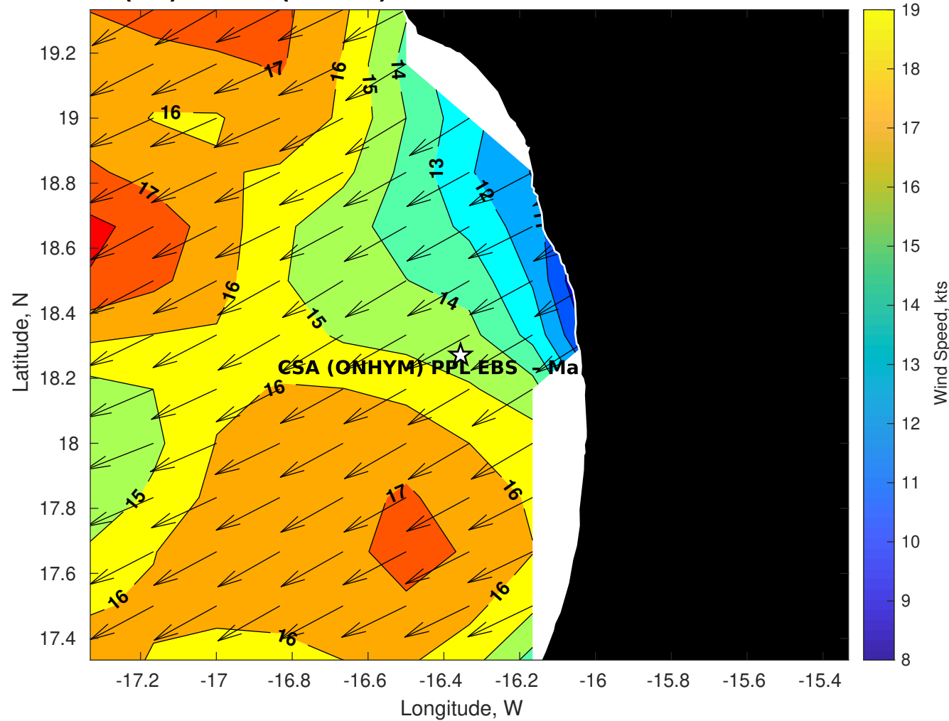
GFS Winds (kts) for CSA (ONHYM) PPL EBS - Mauritania at 19-Dec-2025 09:00:00
