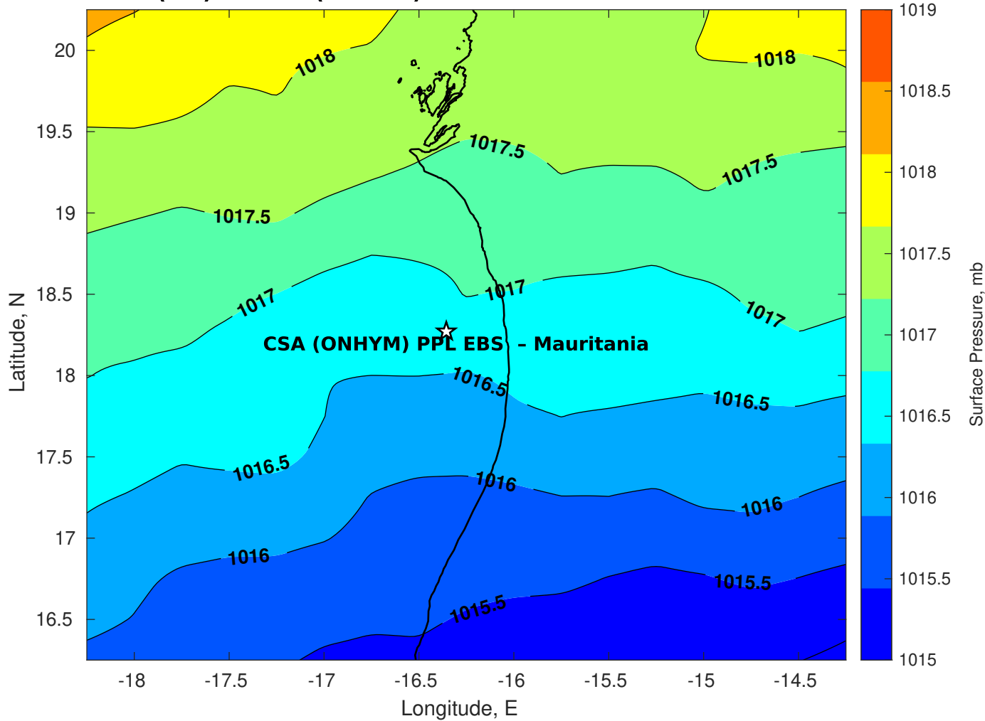
Surface Pressure (mb) for CSA (ONHYM) PPL EBS - Mauritania at 20-Dec-2025 00:00:00
