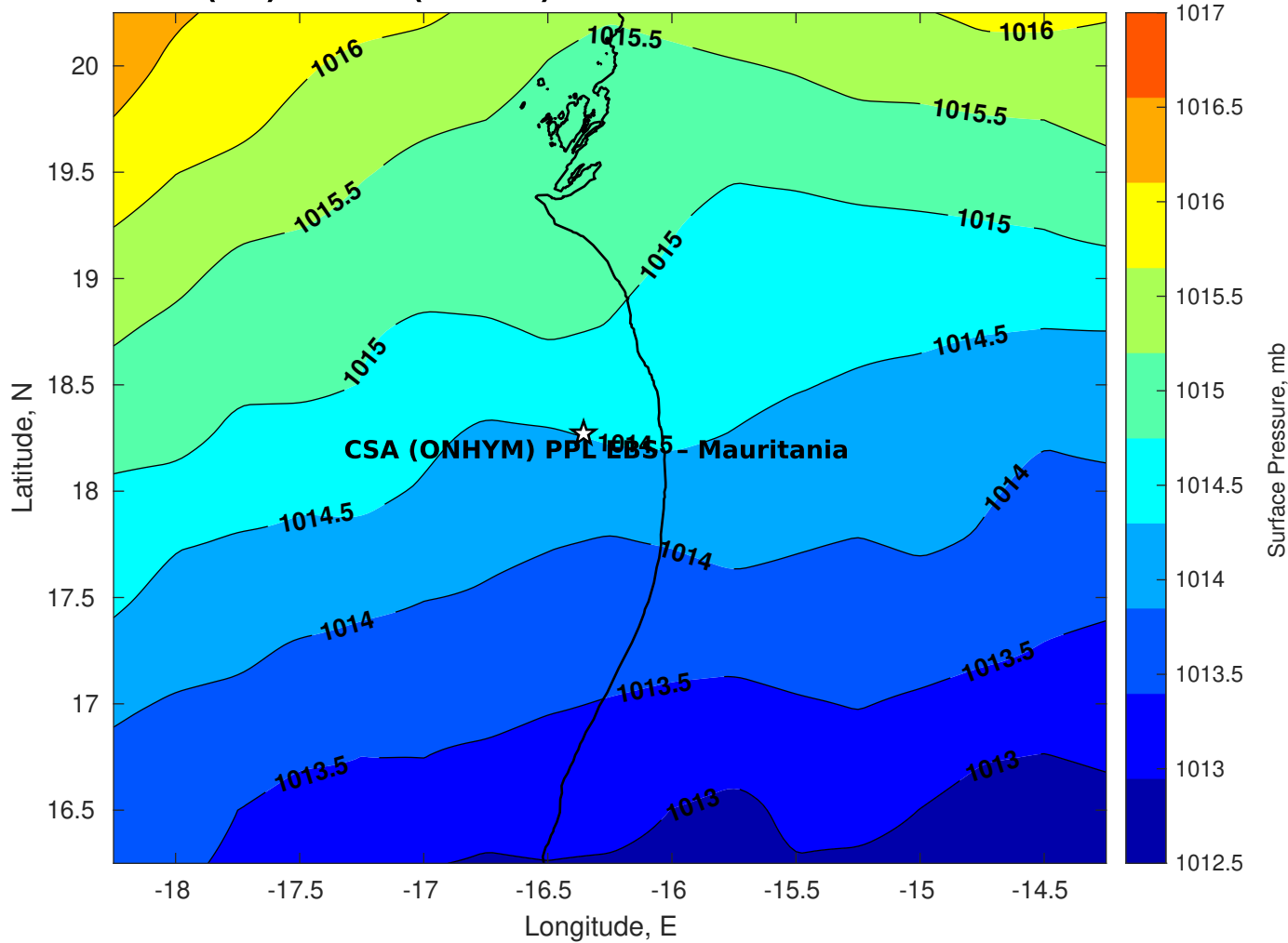
Surface Pressure (mb) for CSA (ONHYM) PPL EBS - Mauritania at 21-Dec-2025 00:00:00
