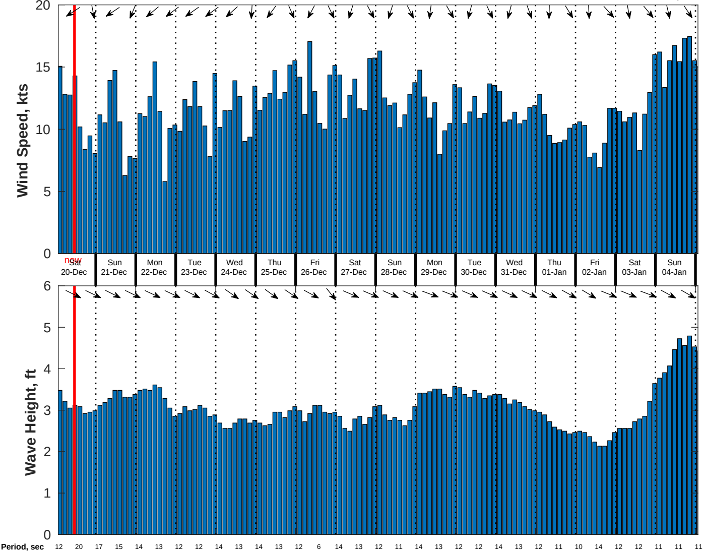
Wind & Wave Forecast for CSA (ONHYM) PPL EBS - Mauritania from 19-Dec-2025 01:00:00 to 04-Jan-2026 01:00:00
