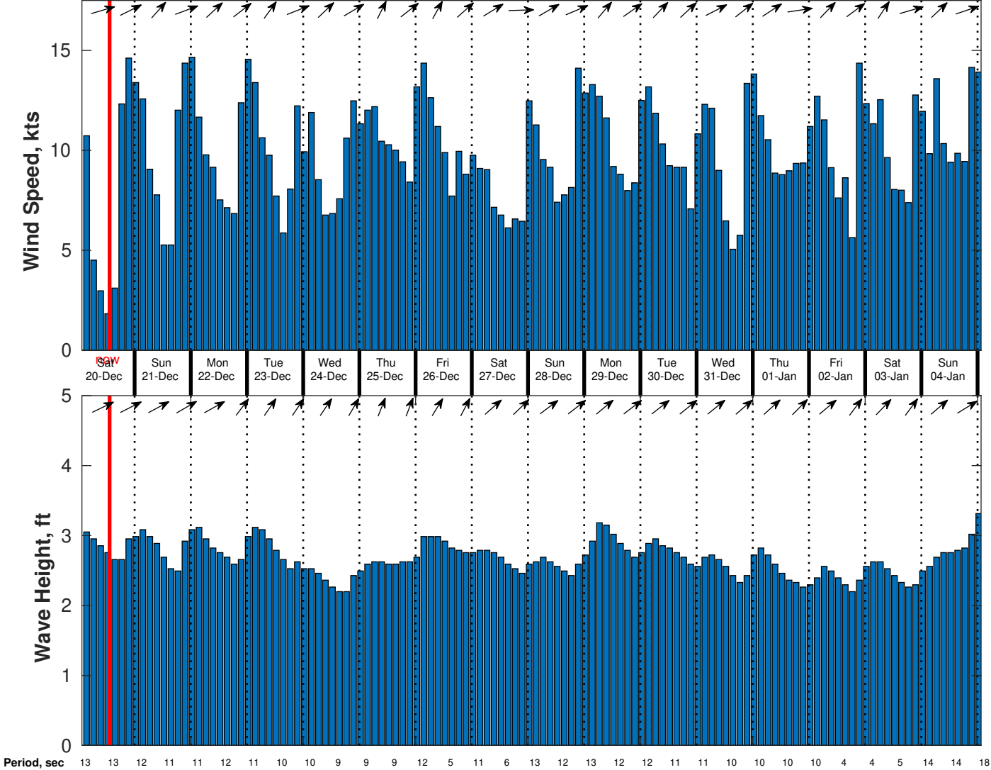
Wind & Wave Forecast for CSA (ONHYM) PPL EBS - Nigeria from 19-Dec-2025 02:00:00 to 04-Jan-2026 02:00:00
