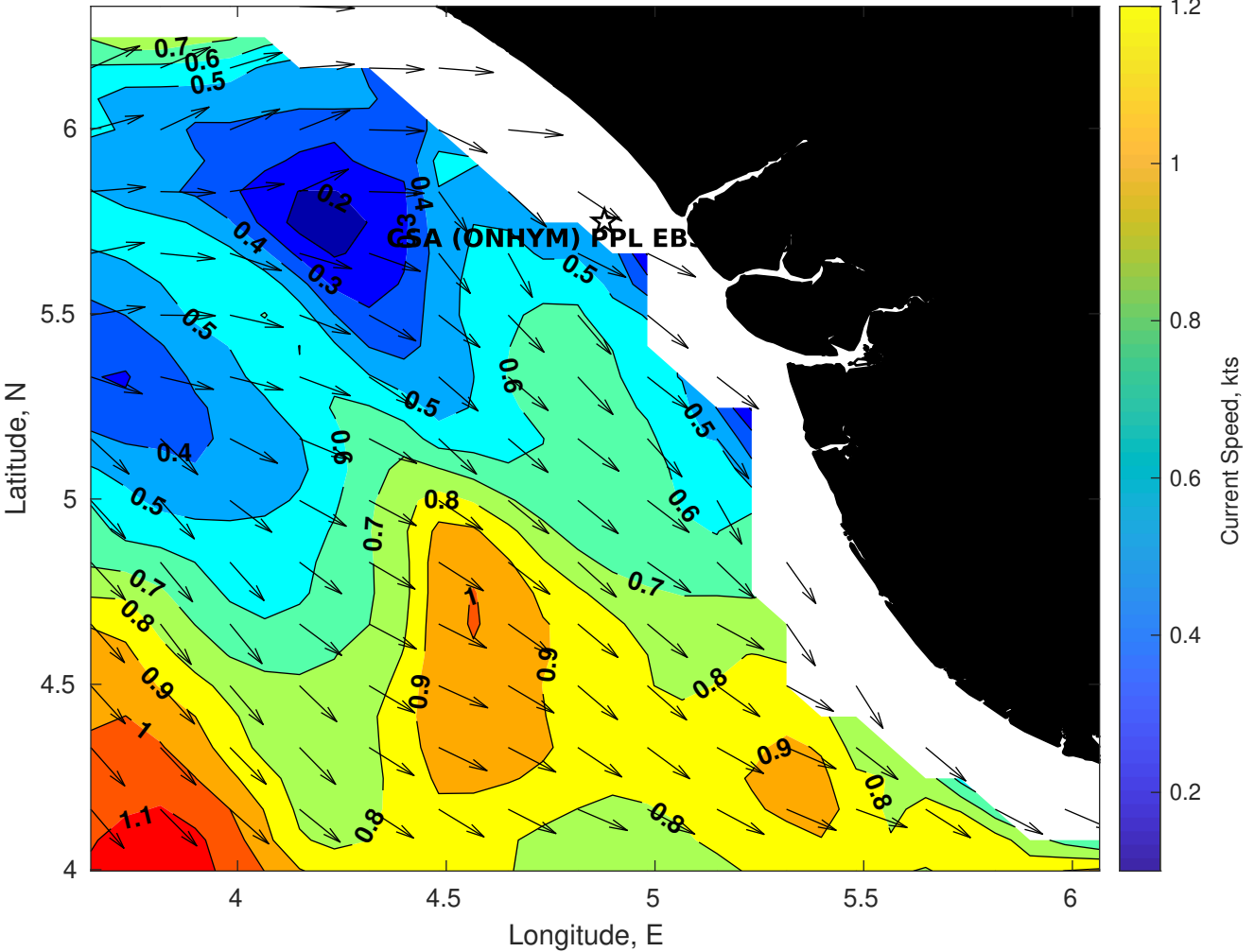
Surface Currents for CSA (ONHYM) PPL EBS - Nigeria at 18-Dec-2025 00:00:00
