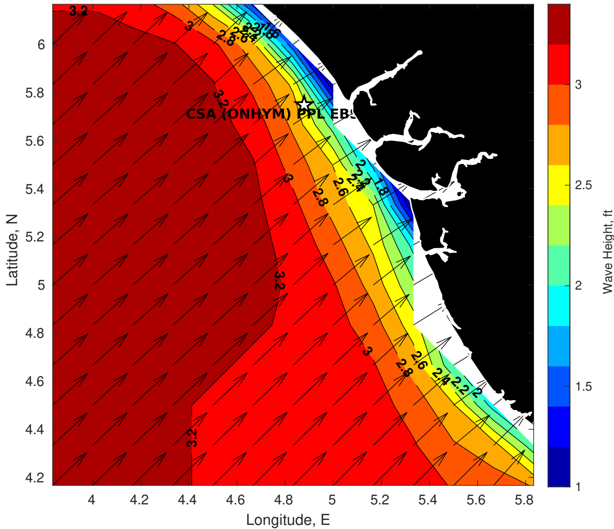
GFS Wave Height (ft) for CSA (ONHYM) PPL EBS - Nigeria at 19-Dec-2025 09:00:00
