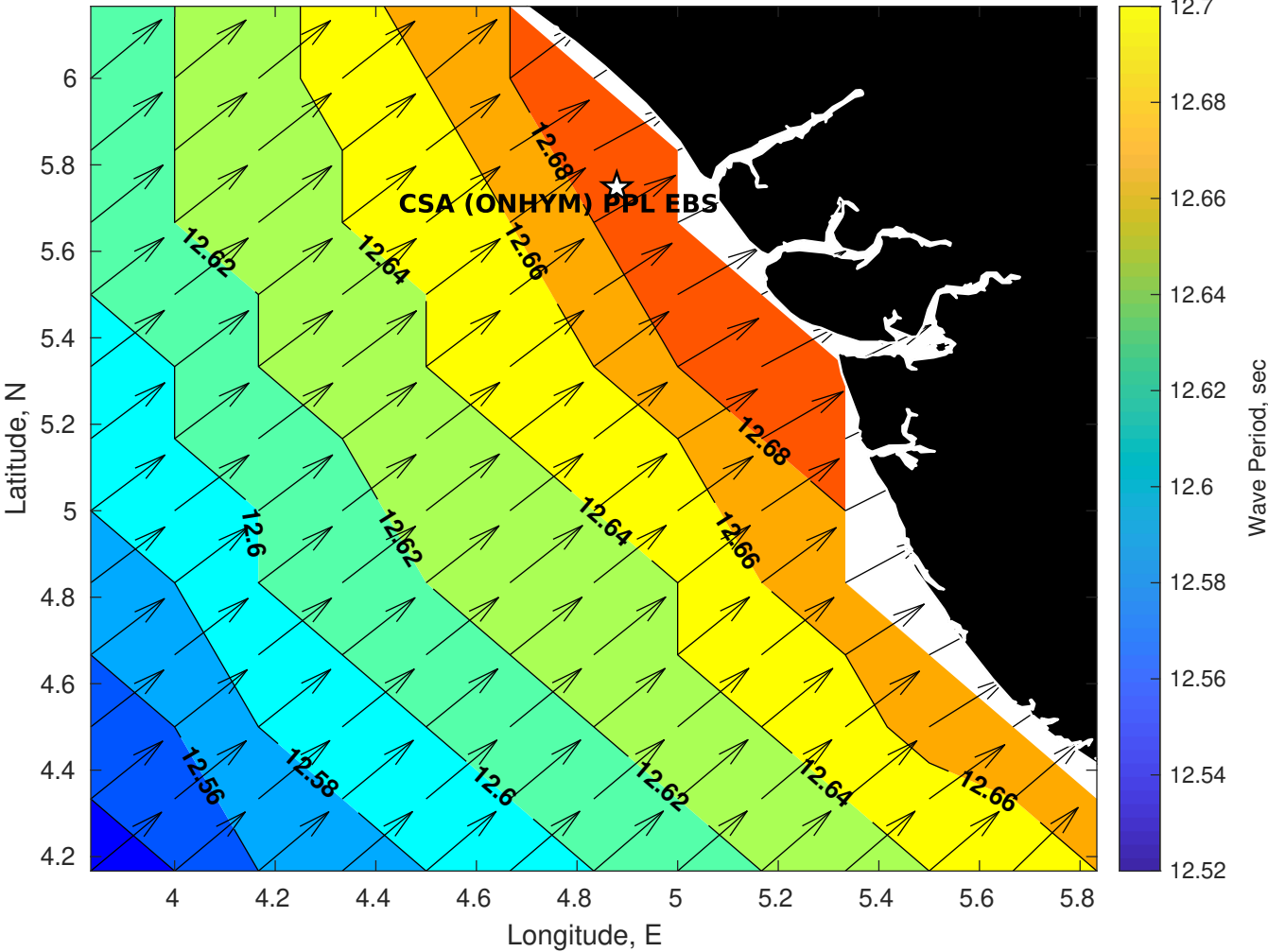
GFS Wave Period (sec) for CSA (ONHYM) PPL EBS - Nigeria at 19-Dec-2025 09:00:00
