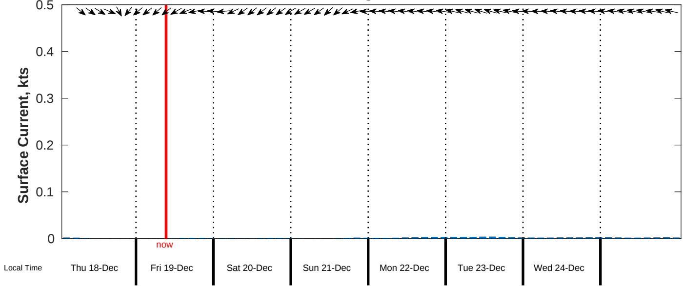
Surface Current Forecast for CSA (ONHYM) PPL EBS - Nigeria from 18-Dec-2025 00:00:00 to 26-Dec-2025 00:00:00
