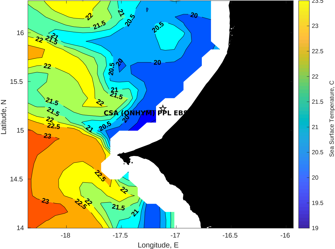
SST for CSA (ONHYM) PPL EBS - Senegal at 18-Dec-2025 00:00:00
