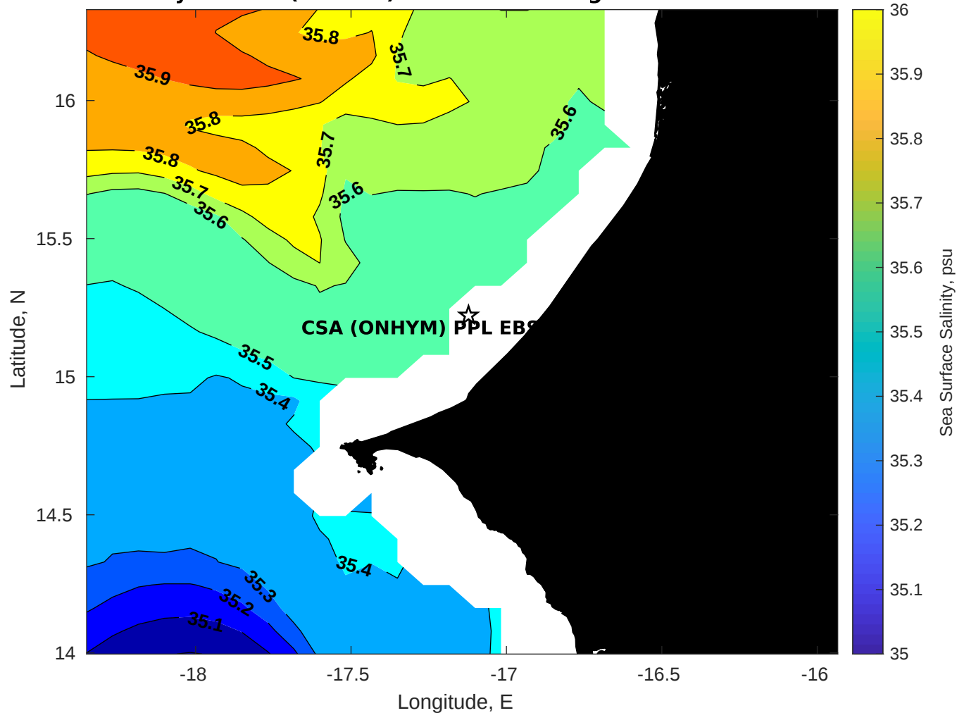
Surface Salinity for CSA (ONHYM) PPL EBS - Senegal at 18-Dec-2025 00:00:00
