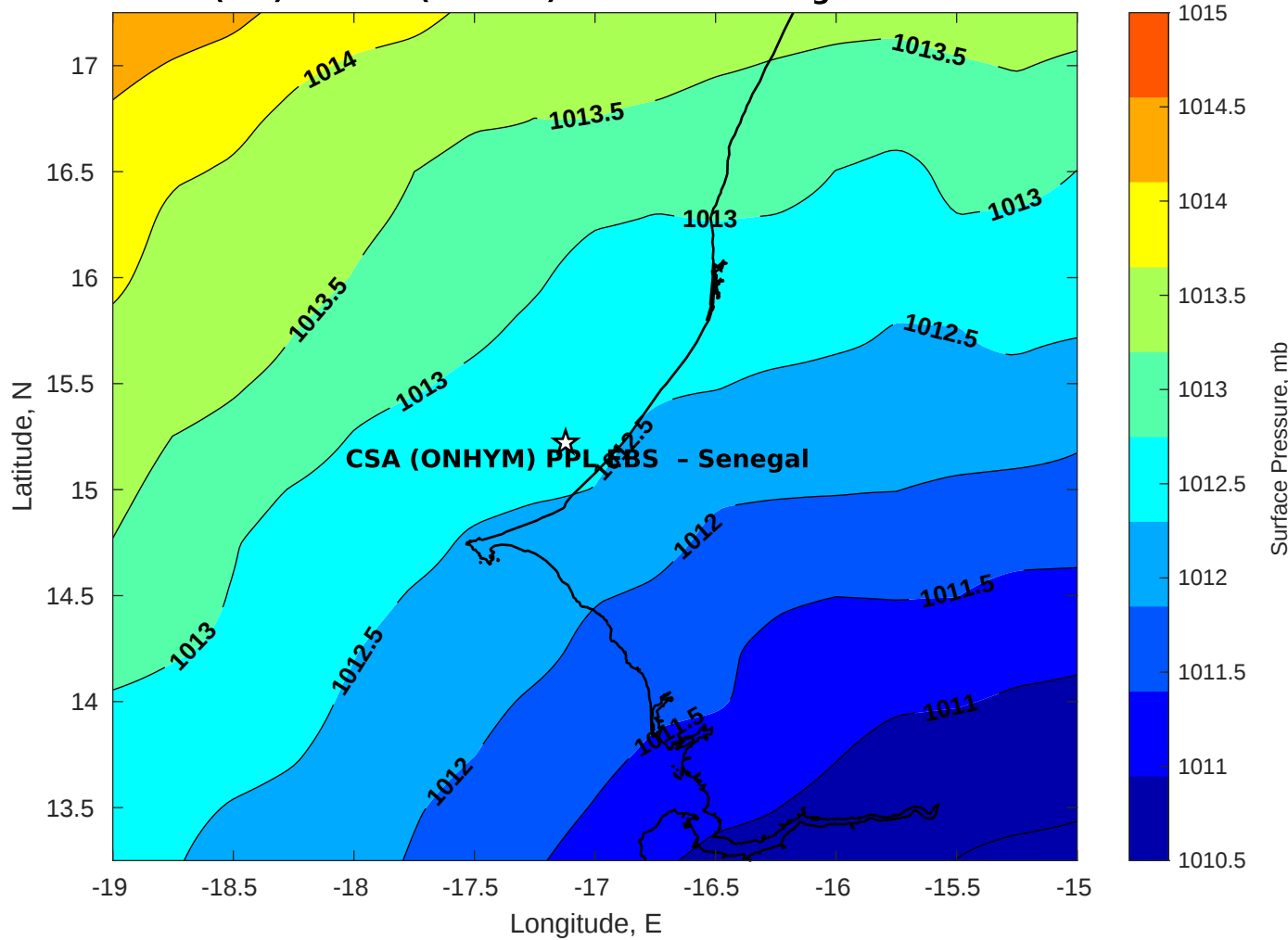
Surface Pressure (mb) for CSA (ONHYM) PPL EBS - Senegal at 21-Dec-2025 00:00:00
