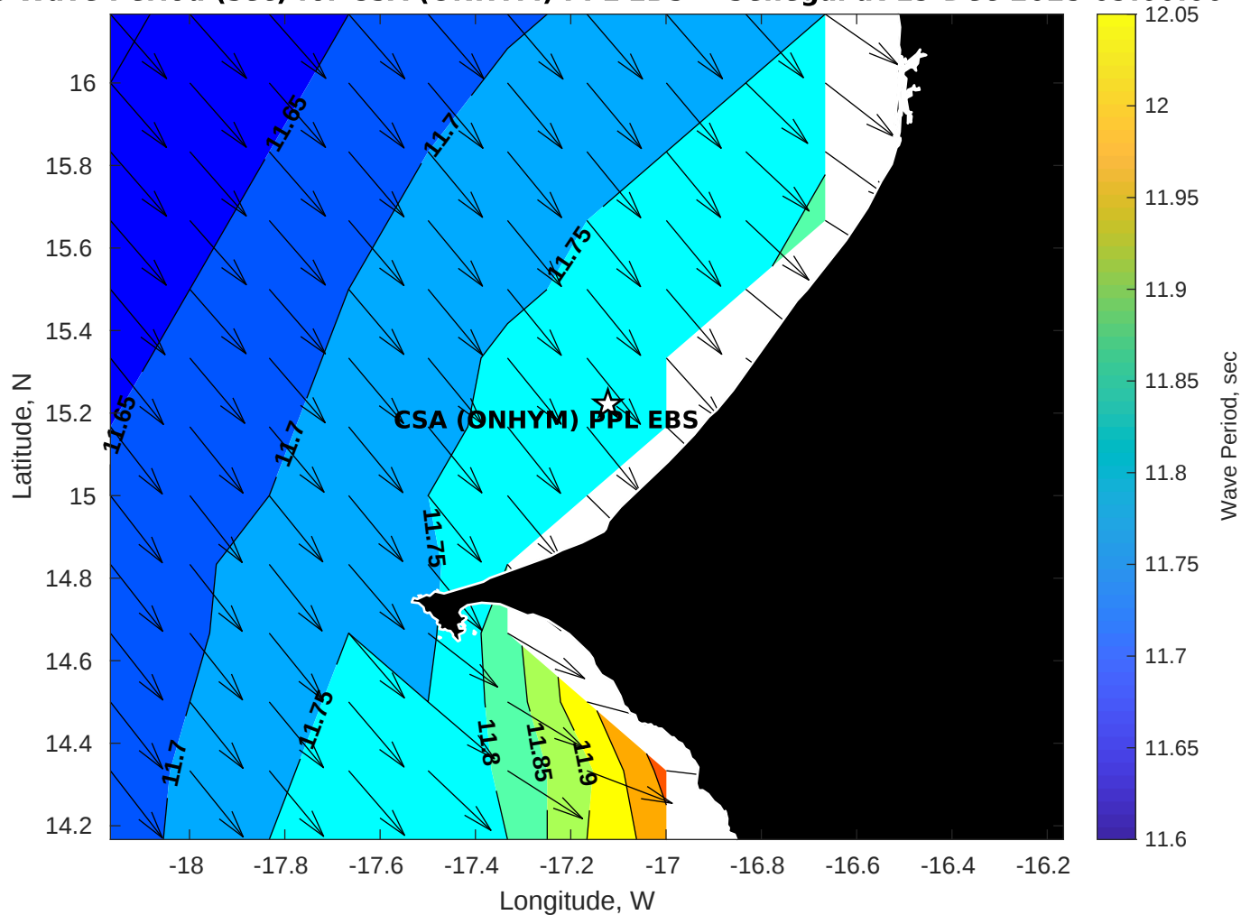
GFS Wave Period (sec) for CSA (ONHYM) PPL EBS - Senegal at 19-Dec-2025 09:00:00
