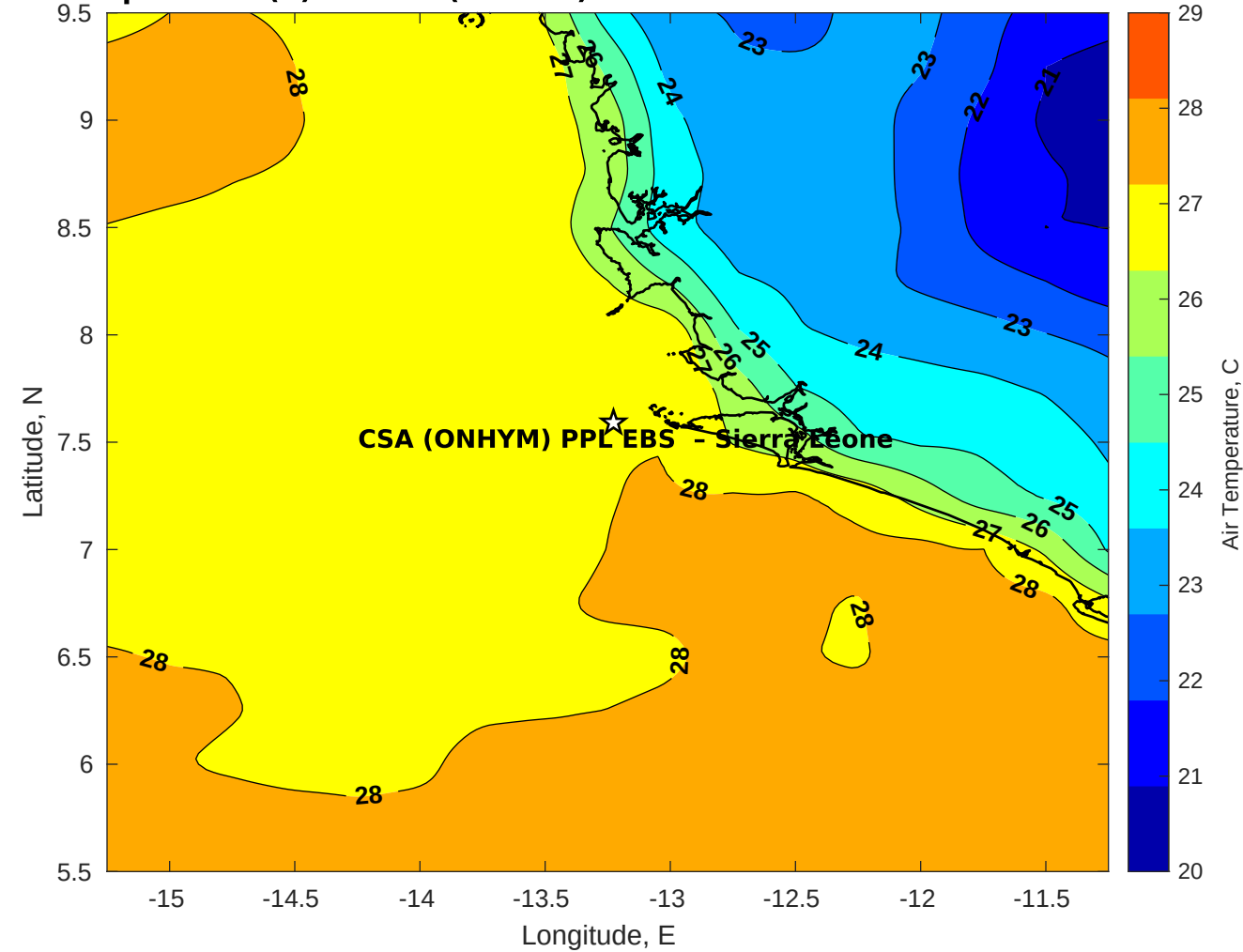
Air Temperature (C) for CSA (ONHYM) PPL EBS - Sierra Leone at 19-Dec-2025
