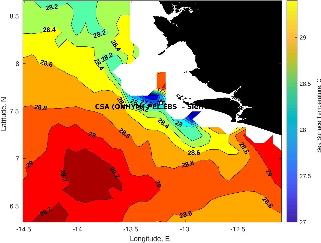
SST for CSA (ONHYM) PPL EBS - Sierra Leone at 18-Dec-2025 00:00:00
