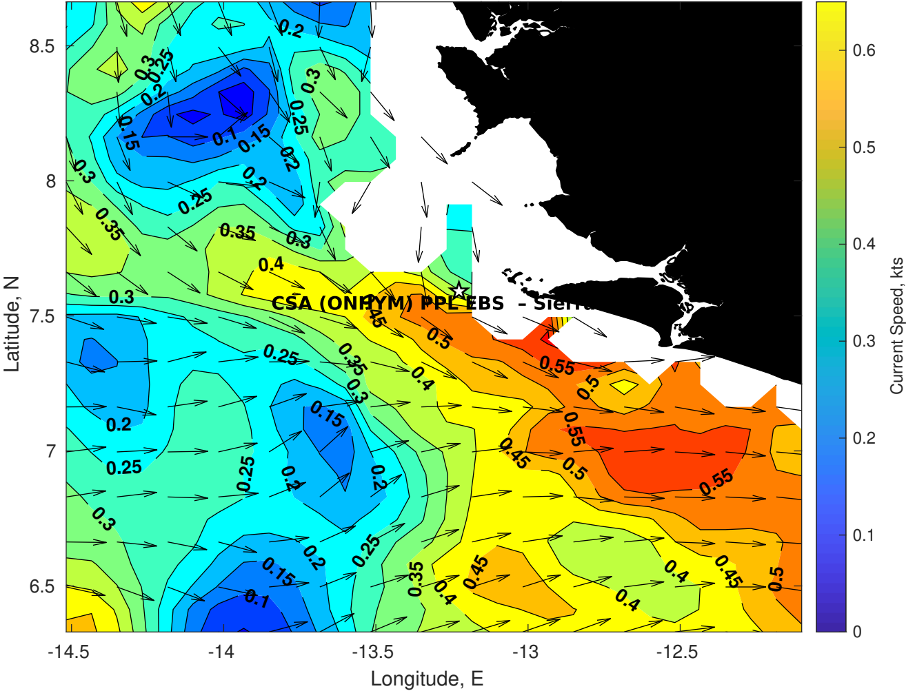
Surface Currents for CSA (ONHYM) PPL EBS - Sierra Leone at 18-Dec-2025 00:00:00
