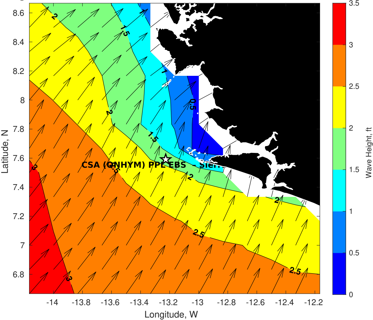
GFS Wave Height (ft) for CSA (ONHYM) PPL EBS - Sierra Leone at 19-Dec-2025 09:00:00
