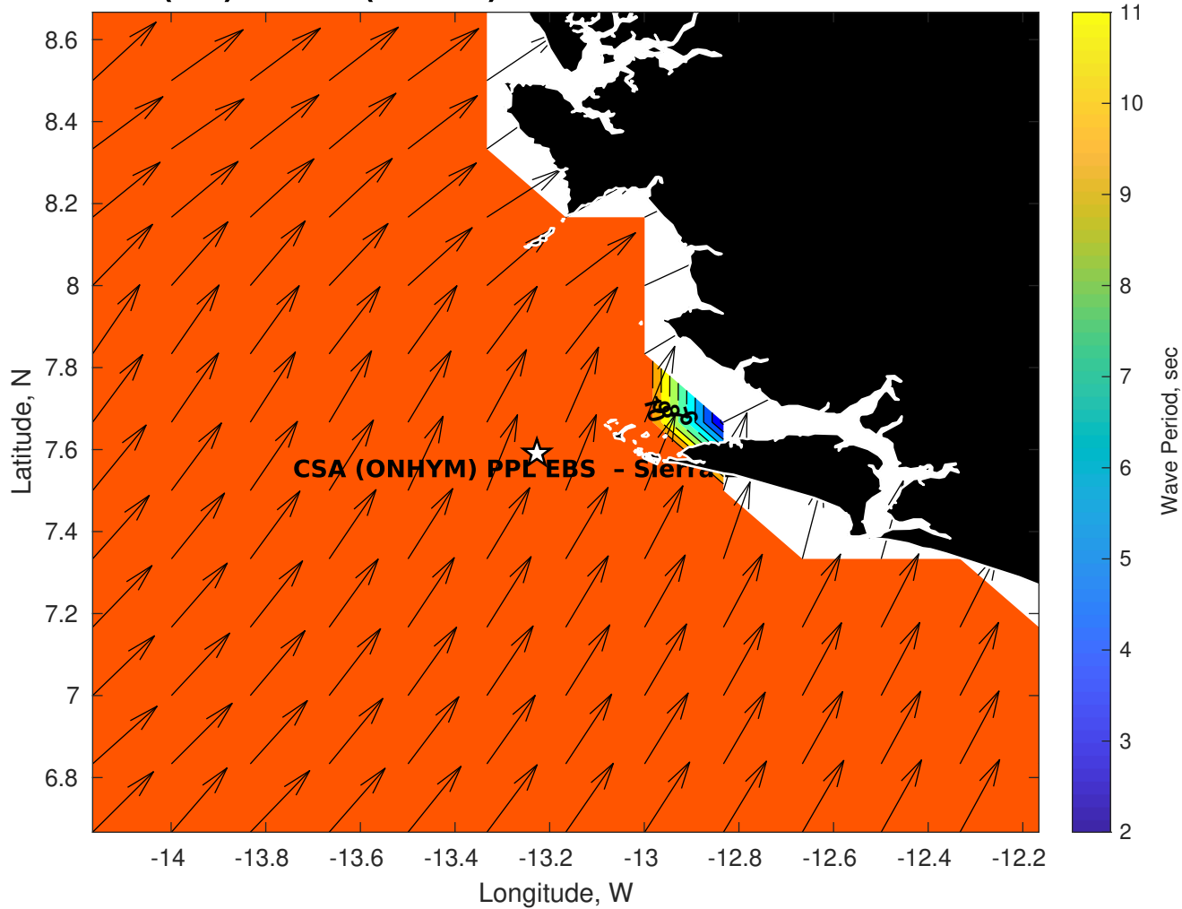
GFS Wave Period (sec) for CSA (ONHYM) PPL EBS - Sierra Leone at 19-Dec-2025 09:00:00
