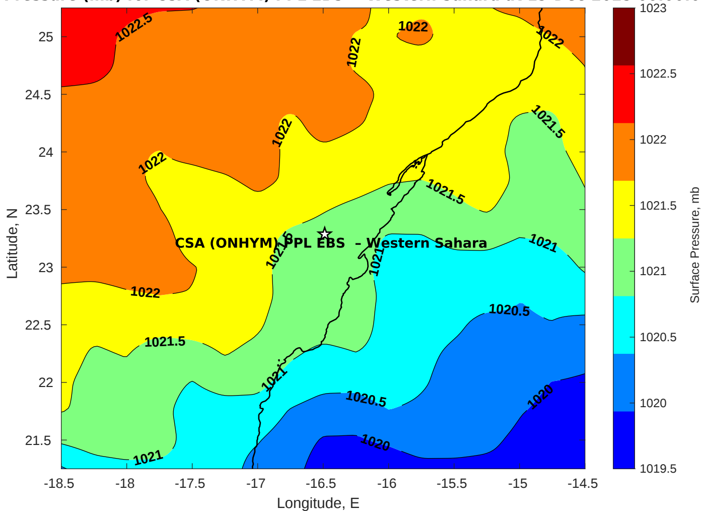
Surface Pressure (mb) for CSA (ONHYM) PPL EBS - Western Sahara at 19-Dec-2025 00:00:00
