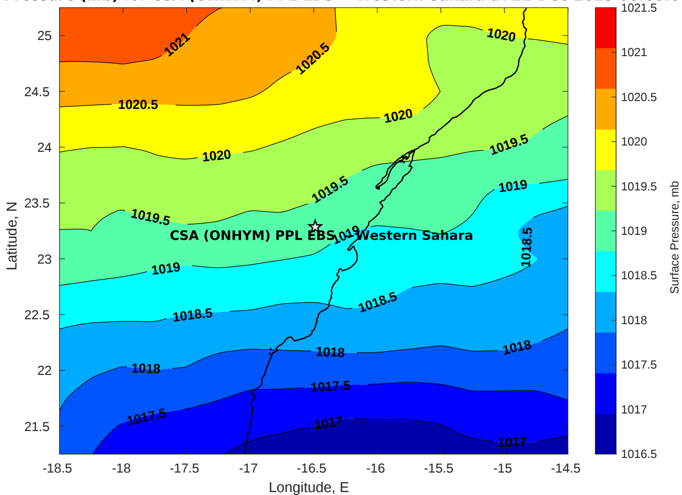
Surface Pressure (mb) for CSA (ONHYM) PPL EBS - Western Sahara at 21-Dec-2025 00:00:00
