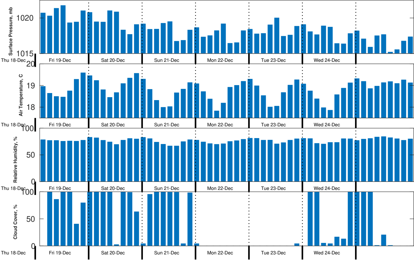
Met Forecast for CSA (ONHYM) PPL EBS - Western Sahara from 19-Dec-2025 00:00:00 to 26-Dec-2025 00:00:00
