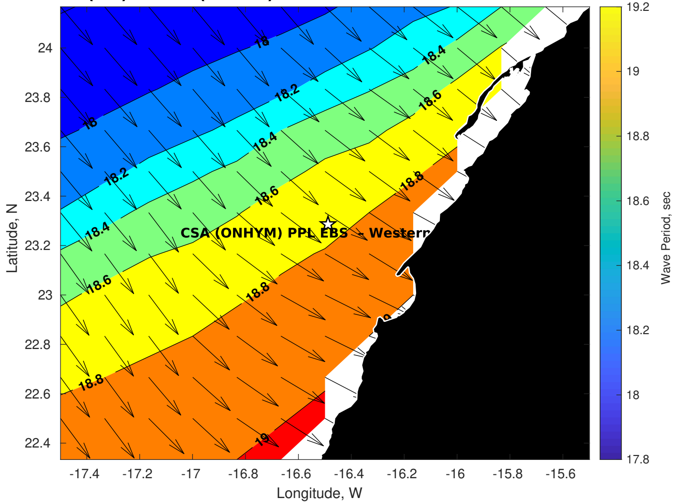
GFS Wave Period (sec) for CSA (ONHYM) PPL EBS - Western Sahara at 19-Dec-2025 09:00:00
