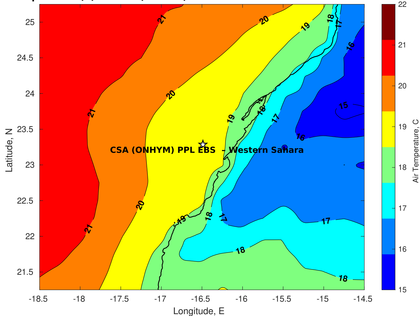
Air Temperature (C) for CSA (ONHYM) PPL EBS - Western Sahara at 19-Dec-2025
