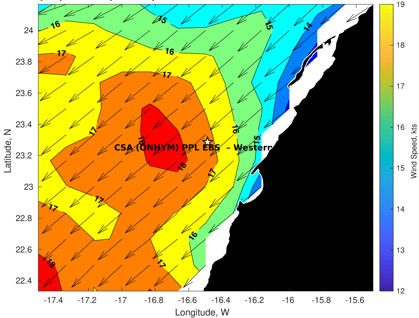
GFS Winds (kts) for CSA (ONHYM) PPL EBS - Western Sahara at 19-Dec-2025 09:00:00
