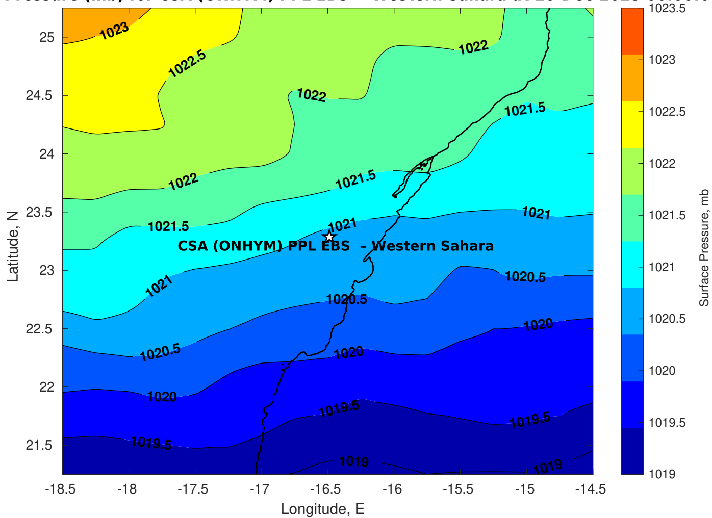
Surface Pressure (mb) for CSA (ONHYM) PPL EBS - Western Sahara at 20-Dec-2025 00:00:00
