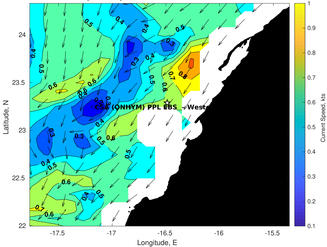
Surface Currents for CSA (ONHYM) PPL EBS - Western Sahara at 18-Dec-2025 00:00:00
