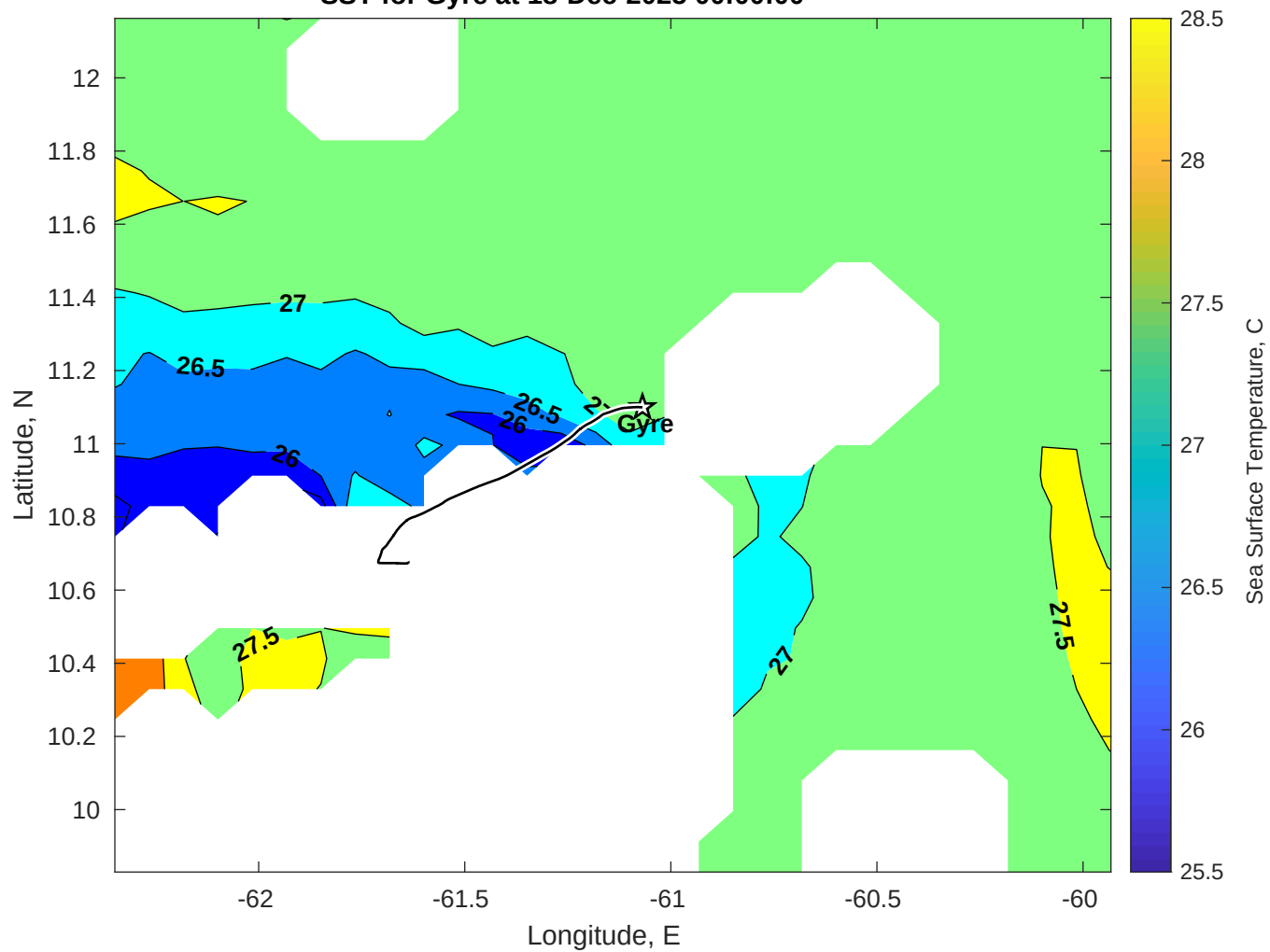
SST for Gyre at 18-Dec-2025 00:00:00
