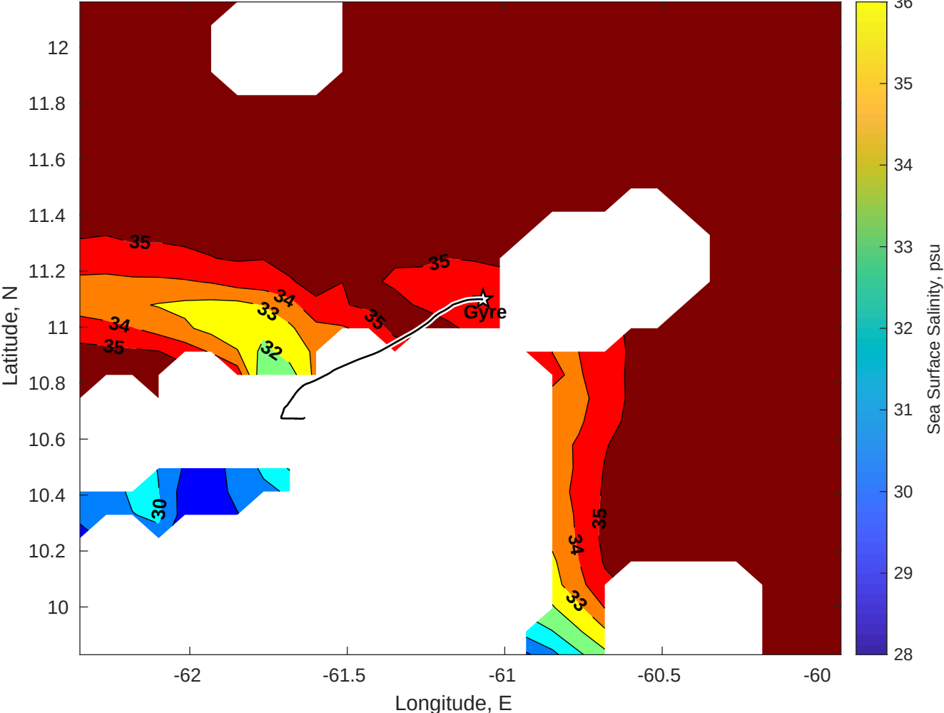
Surface Salinity for Gyre at 18-Dec-2025 00:00:00
