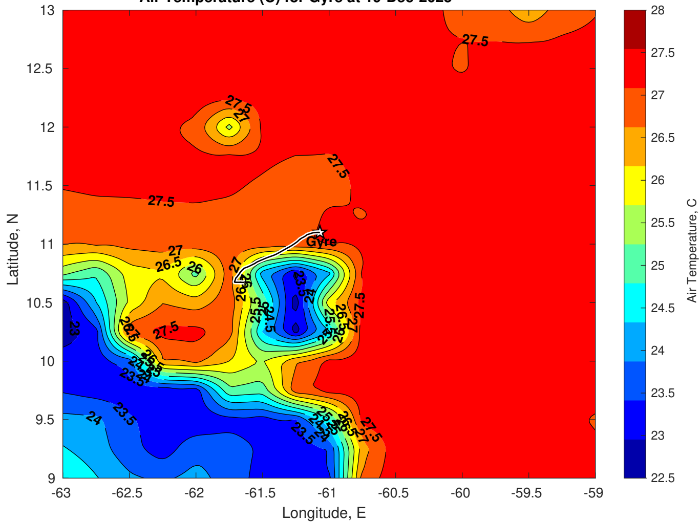
Air Temperature (C) for Gyre at 19-Dec-2025
