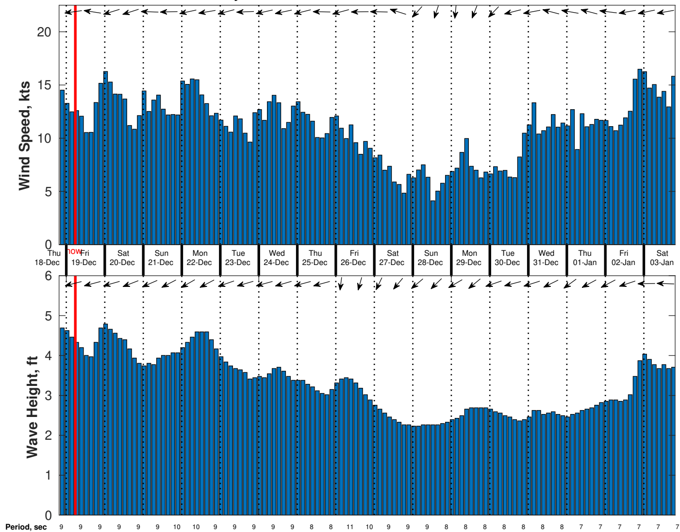
Wind & Wave Forecast for Gyre from 18-Dec-2025 20:00:00 to 03-Jan-2026 20:00:00
