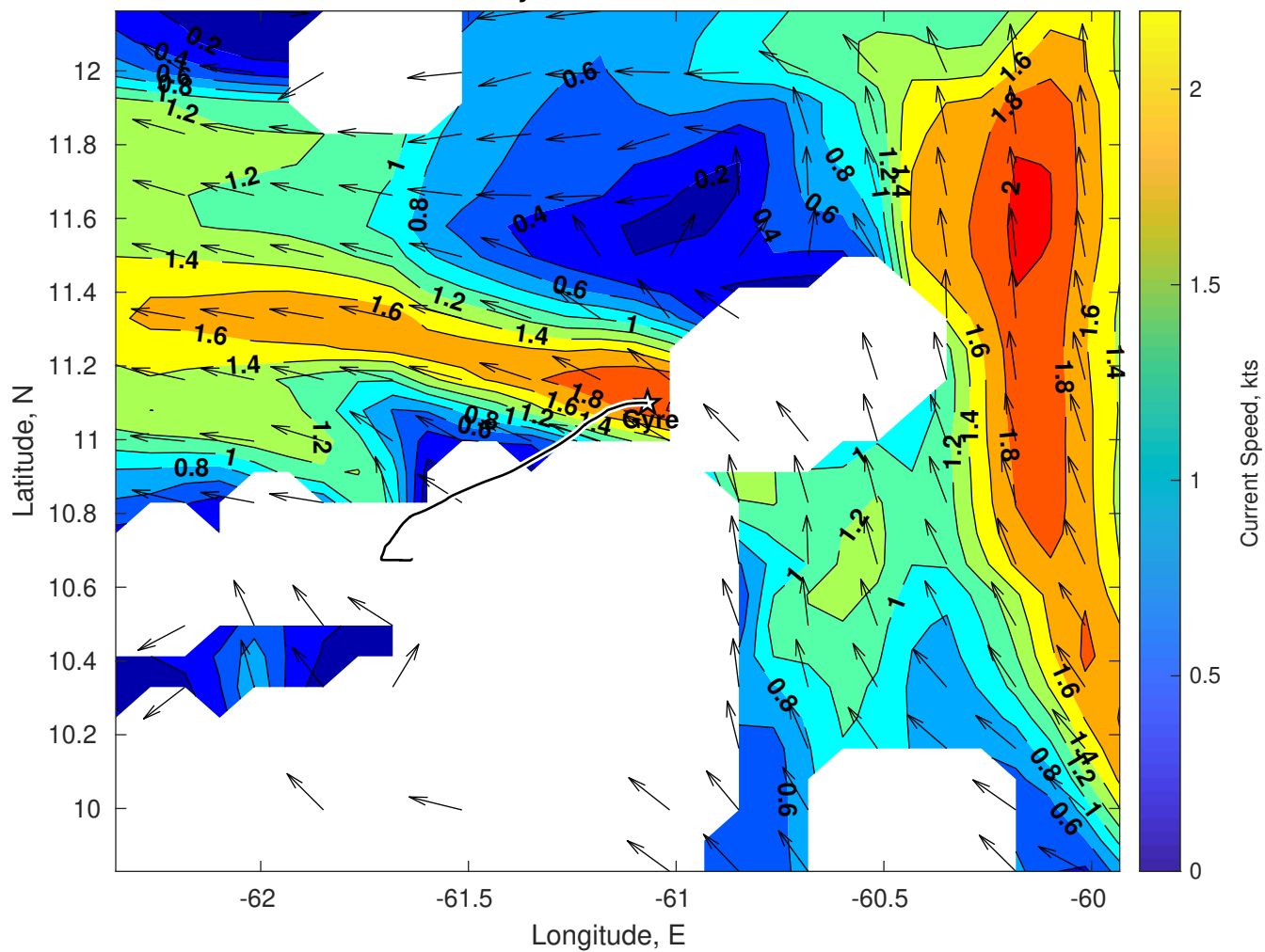
Surface Currents for Gyre at 18-Dec-2025 00:00:00
