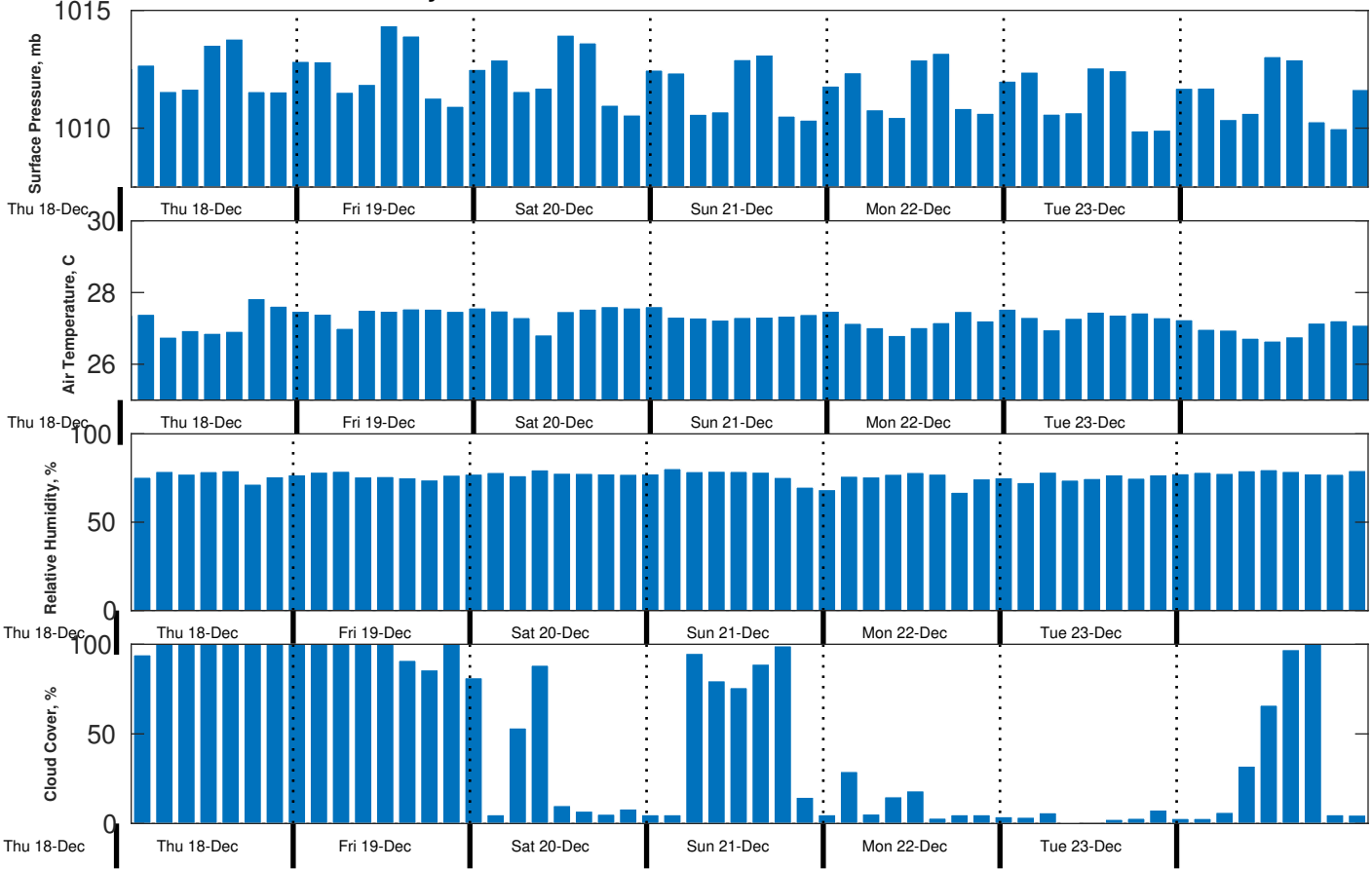
Met Forecast for Gyre from 18-Dec-2025 20:00:00 to 25-Dec-2025 20:00:00
