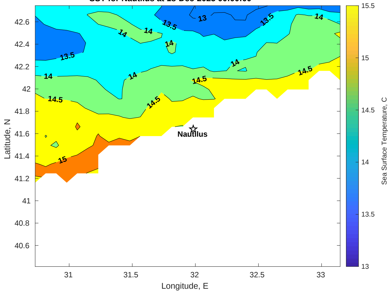
SST for Nautilus at 18-Dec-2025 00:00:00
