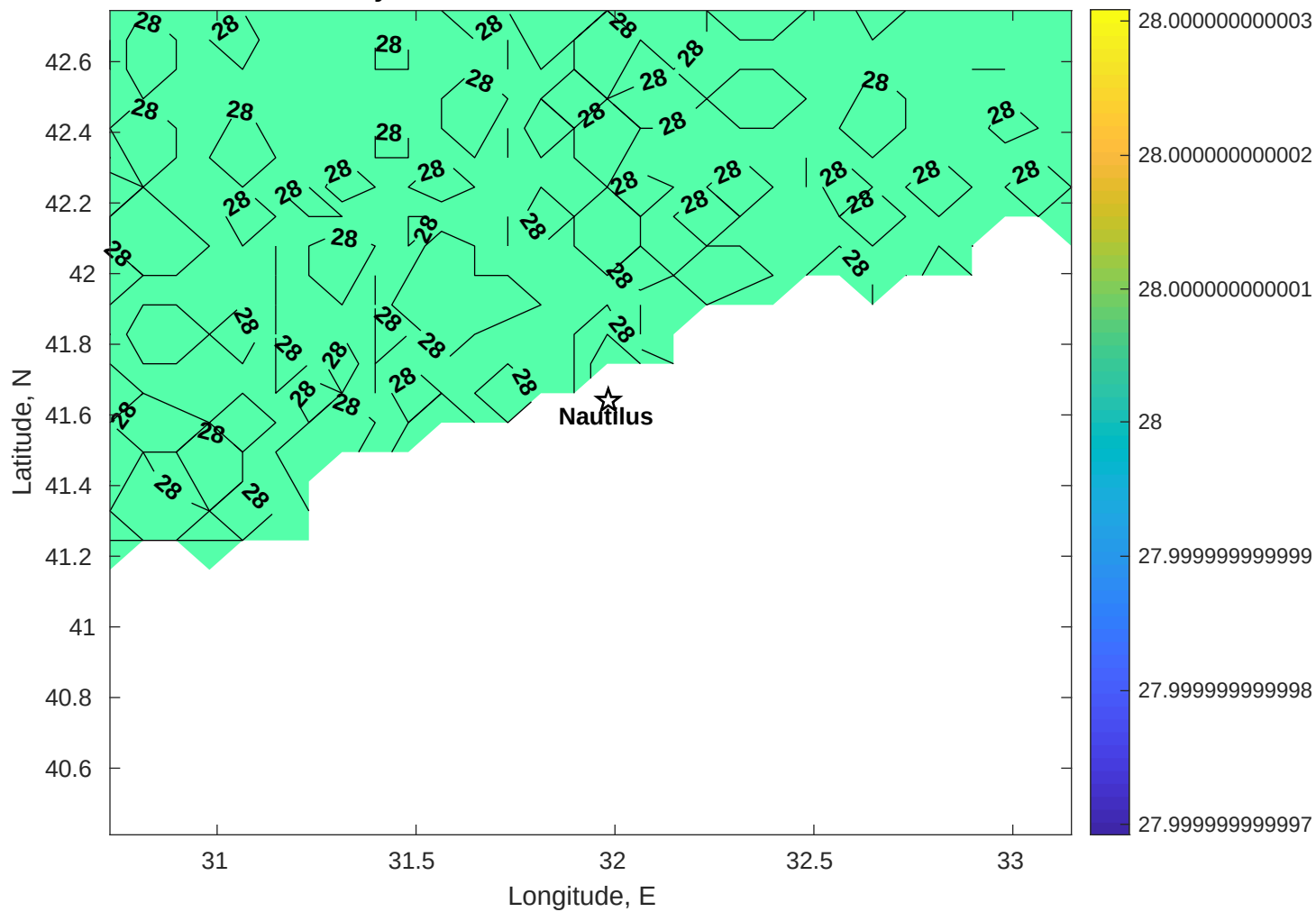
Surface Salinity for Nautilus at 18-Dec-2025 00:00:00
