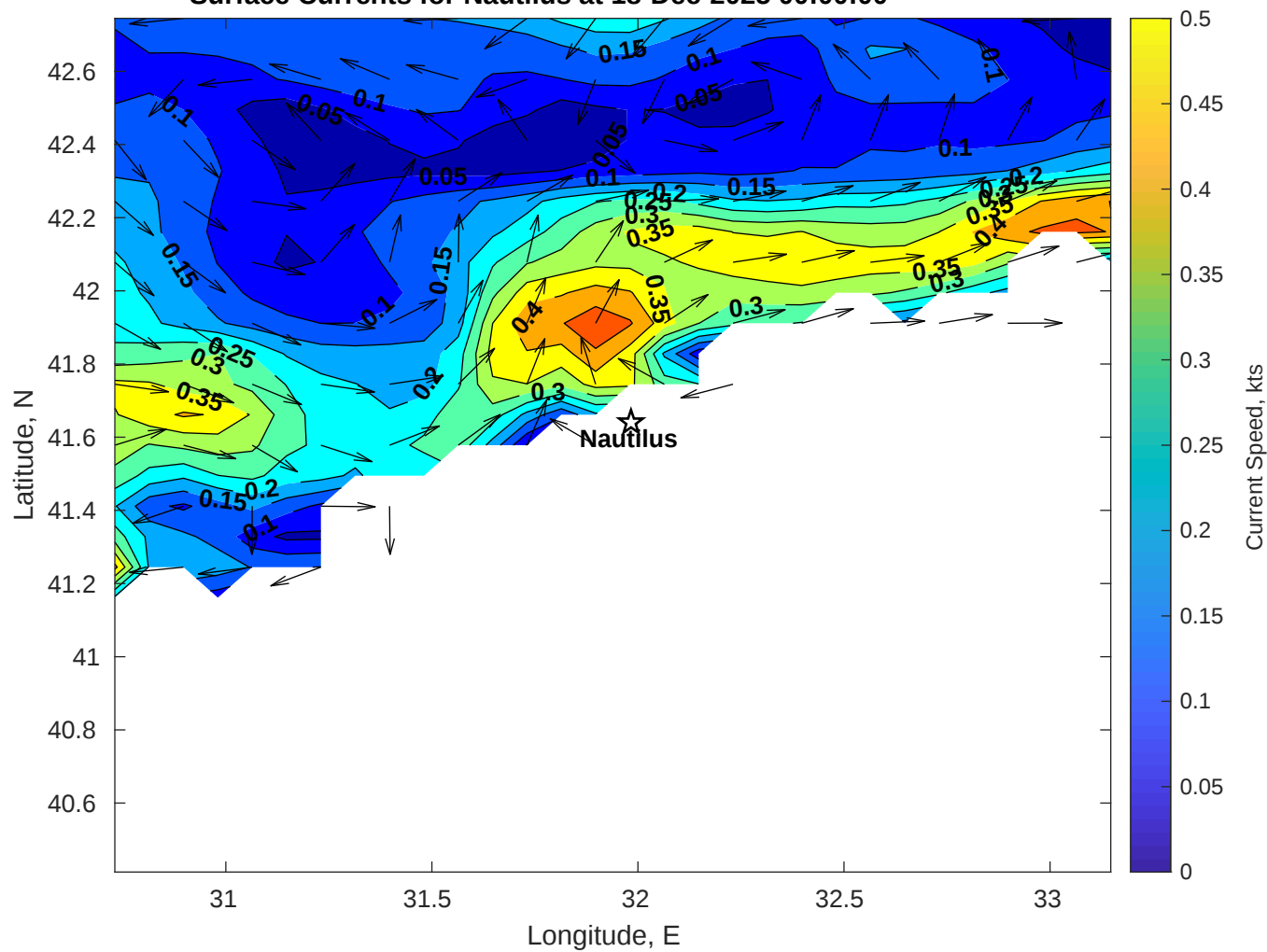
Surface Currents for Nautilus at 18-Dec-2025 00:00:00
