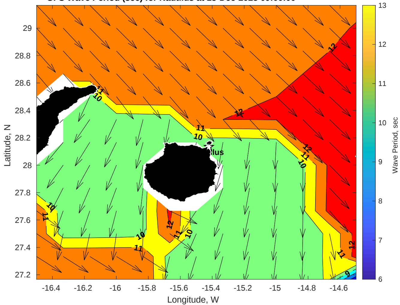
GFS Wave Period (sec) for Nautilus at 18-Dec-2025 09:00:00
