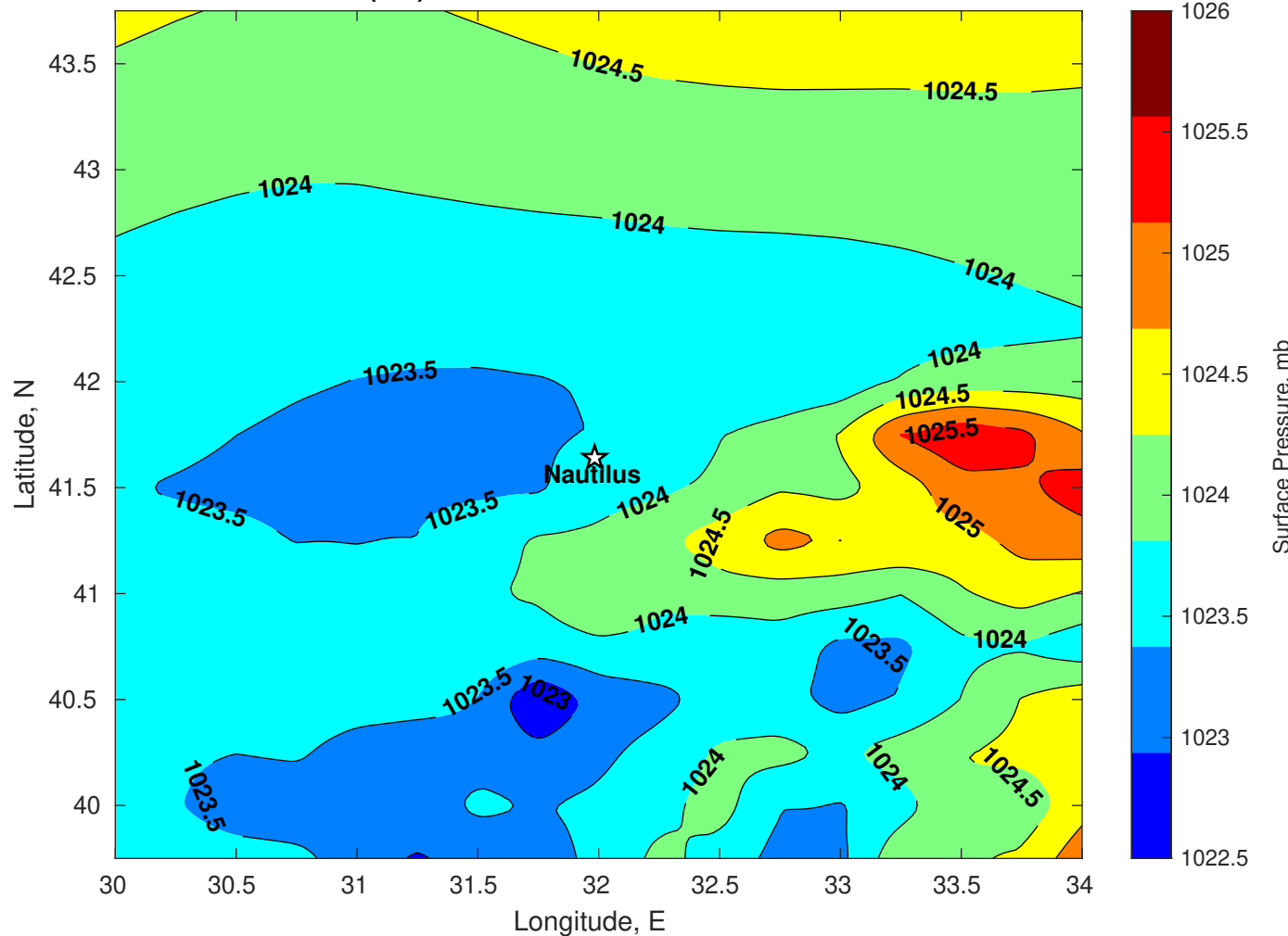
Surface Pressure (mb) for Nautilus at 20-Dec-2025 00:00:00
