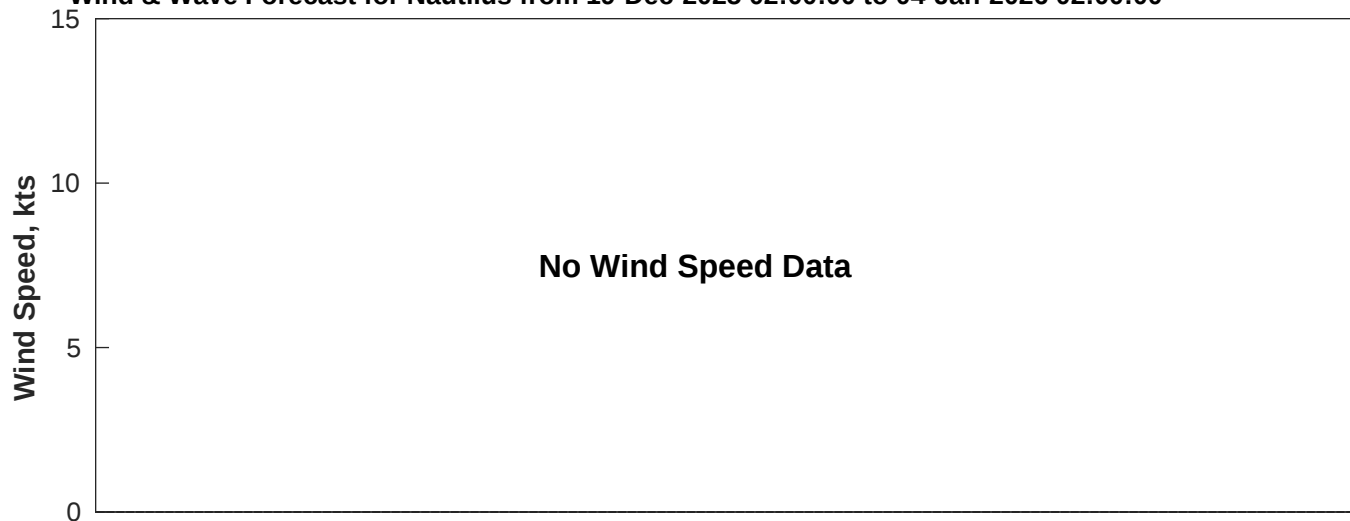
Wind & Wave Forecast for Nautilus from 19-Dec-2025 02:00:00 to 04-Jan-2026 02:00:00
