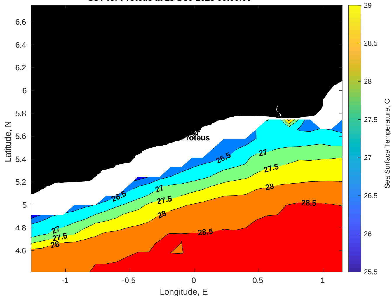
SST for Proteus at 18-Dec-2025 00:00:00
