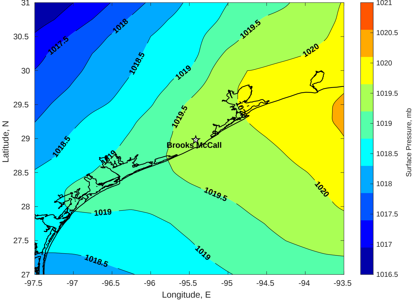
Surface Pressure (mb) for Brooks McCall at 20-Dec-2025 00:00:00
