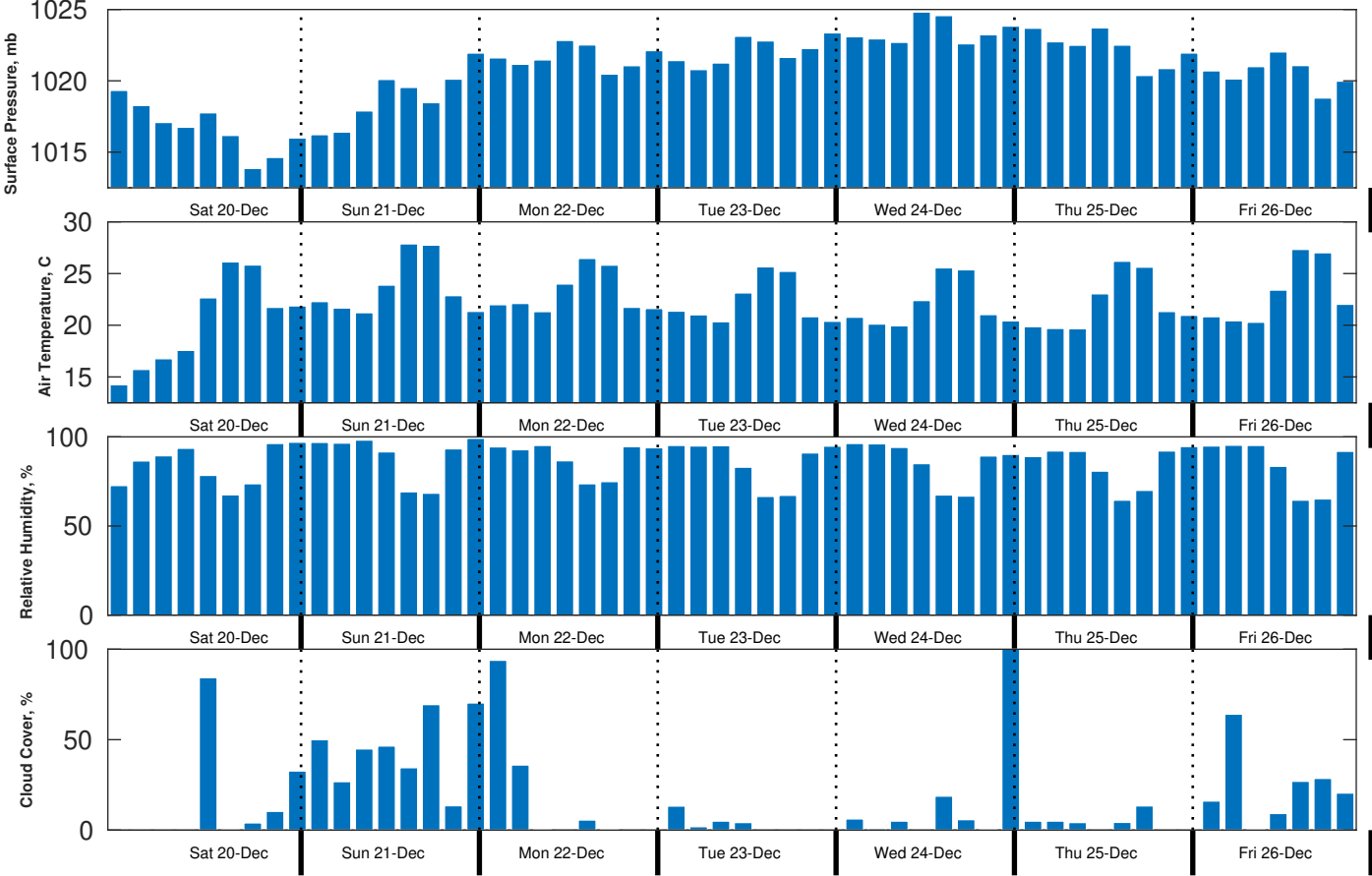
Met Forecast for Brooks McCall from 20-Dec-2025 00:00:00 to 27-Dec-2025 00:00:00
