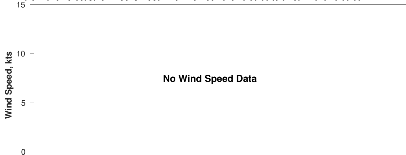
Wind & Wave Forecast for Brooks McCall from 19-Dec-2025 20:00:00 to 04-Jan-2026 20:00:00
