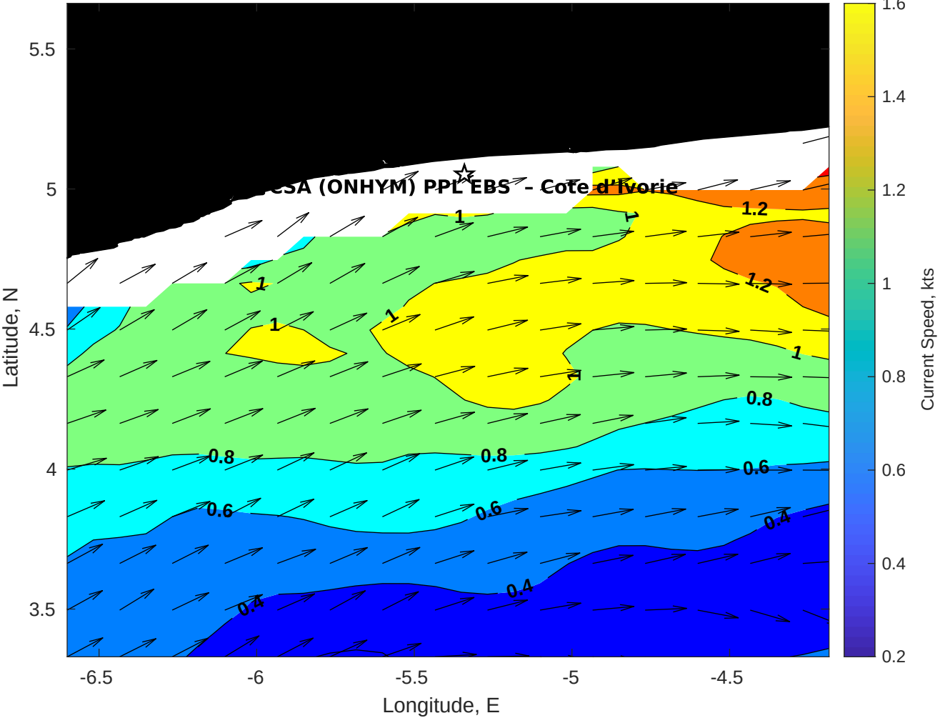
Surface Currents for CSA (ONHYM) PPL EBS - Cote d'Ivoire at 19-Dec-2025 00:00:00
