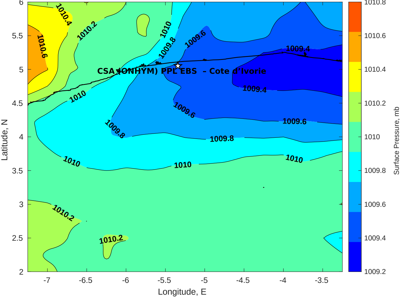
Surface Pressure (mb) for CSA (ONHYM) PPL EBS - Cote d'Ivoire at 22-Dec-2025 00:00:00
