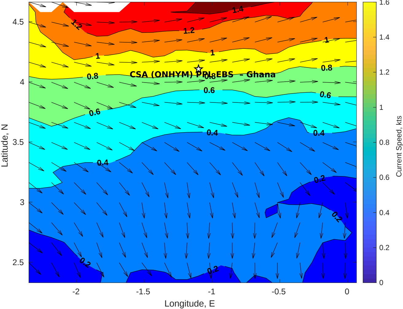
Surface Currents for CSA (ONHYM) PPL EBS - Ghana at 19-Dec-2025 00:00:00
