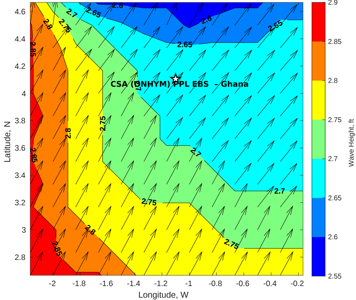
GFS Wave Height (ft) for CSA (ONHYM) PPL EBS - Ghana at 20-Dec-2025 09:00:00
