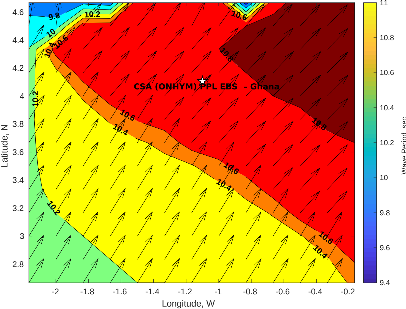
GFS Wave Period (sec) for CSA (ONHYM) PPL EBS - Ghana at 20-Dec-2025 09:00:00
