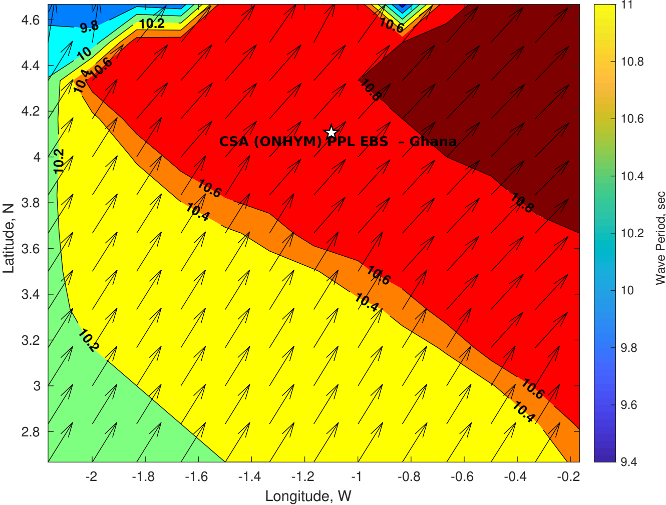
GFS Wave Period (sec) for CSA (ONHYM) PPL EBS - Ghana at 20-Dec-2025 09:00:00
