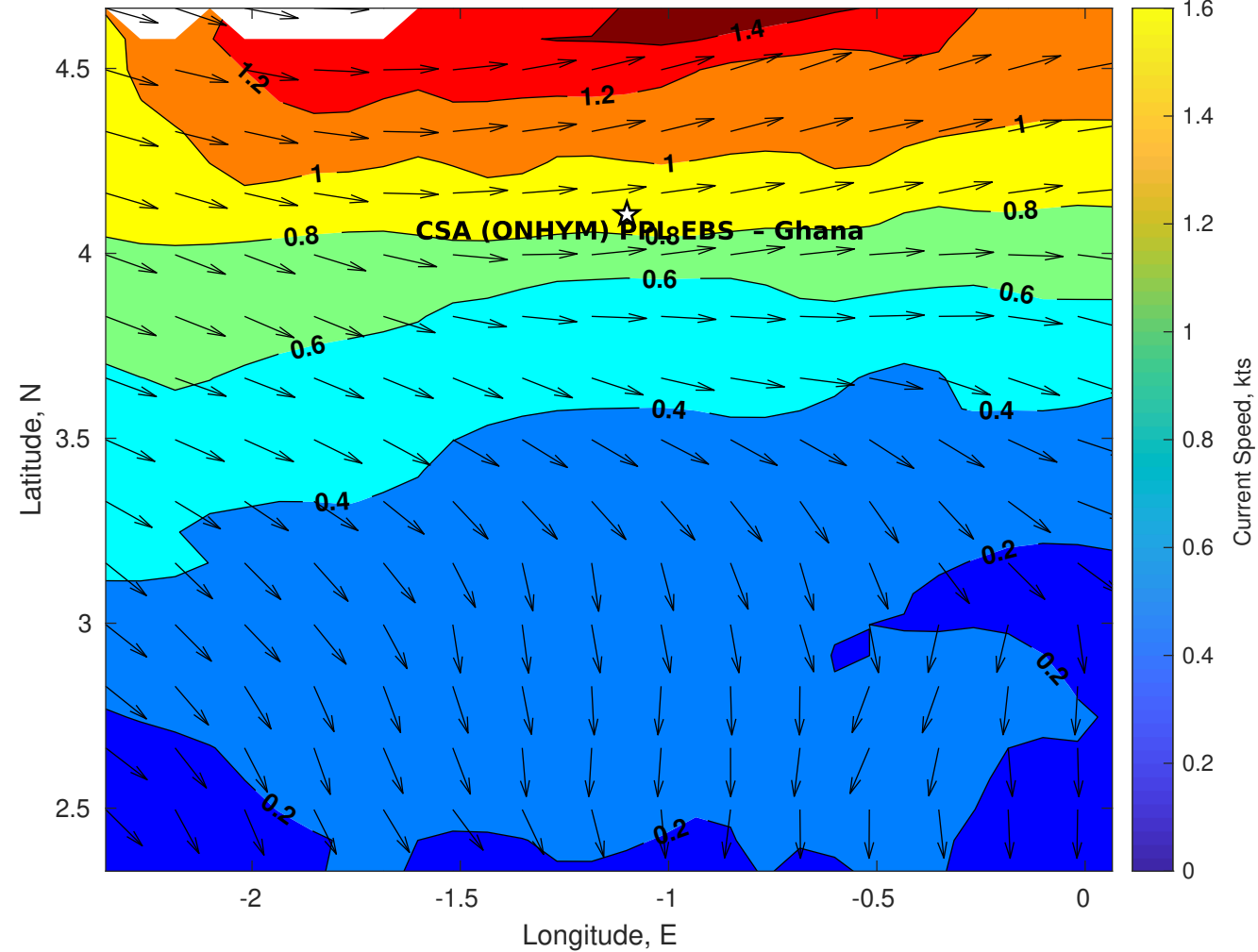
Surface Currents for CSA (ONHYM) PPL EBS - Ghana at 19-Dec-2025 00:00:00
