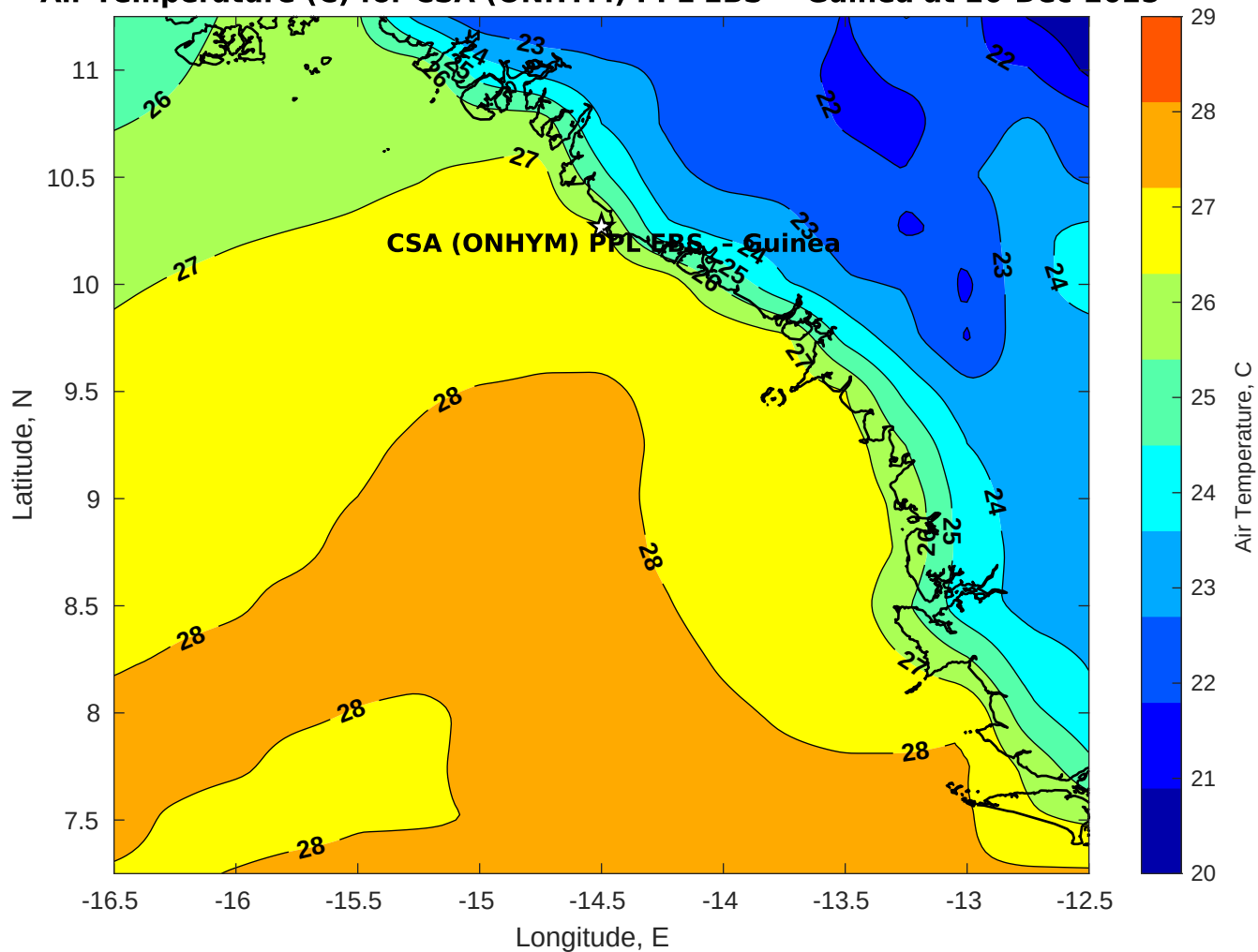
Air Temperature (C) for CSA (ONHYM) PPL EBS - Guinea at 20-Dec-2025
