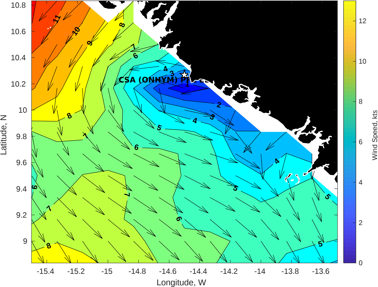
GFS Winds (kts) for CSA (ONHYM) PPL EBS - Guinea at 20-Dec-2025 09:00:00
