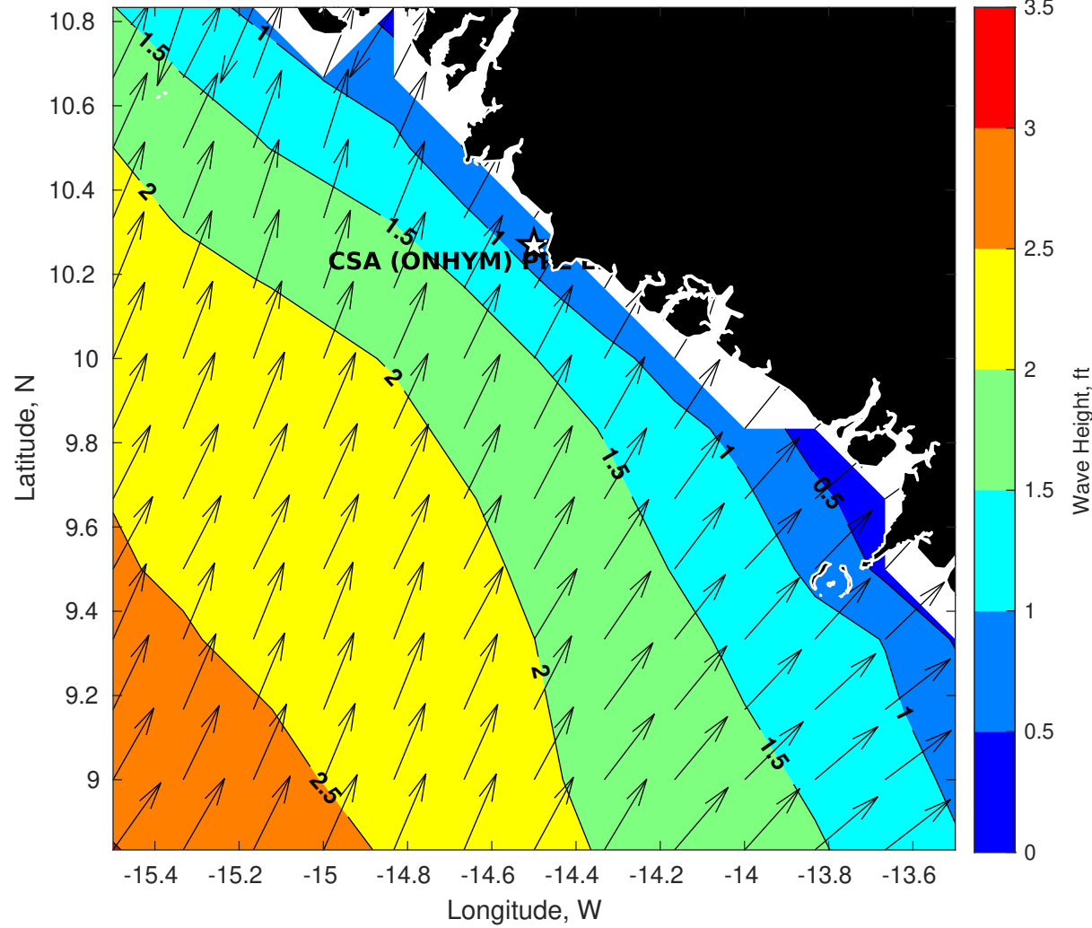
GFS Wave Height (ft) for CSA (ONHYM) PPL EBS - Guinea at 20-Dec-2025 09:00:00
