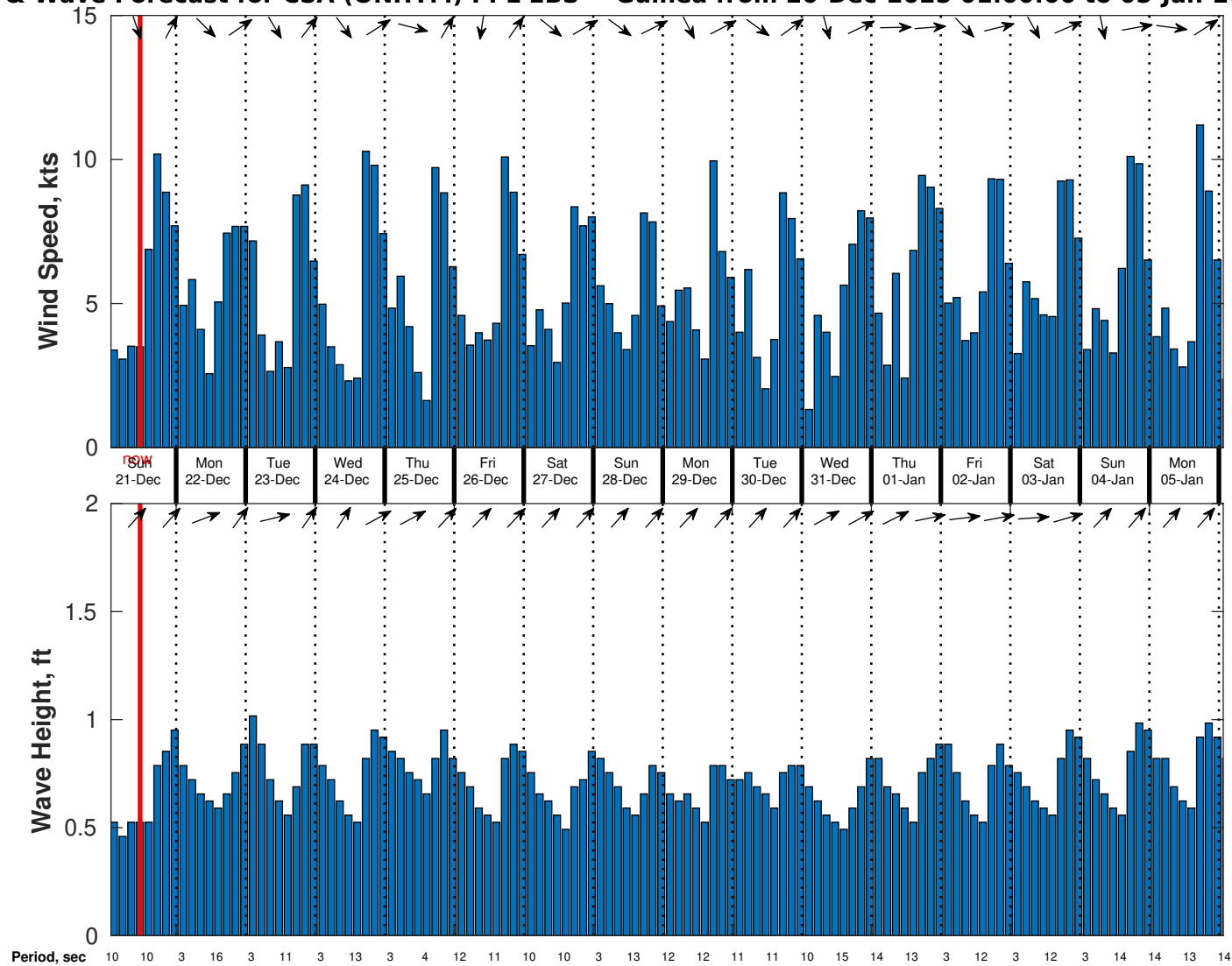
Wind & Wave Forecast for CSA (ONHYM) PPL EBS - Guinea from 20-Dec-2025 01:00:00 to 05-Jan-2026 01:00:00
