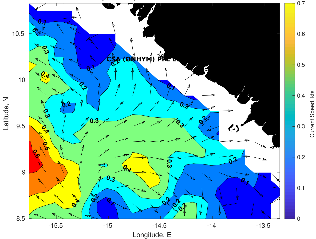
Surface Currents for CSA (ONHYM) PPL EBS - Guinea at 19-Dec-2025 00:00:00
