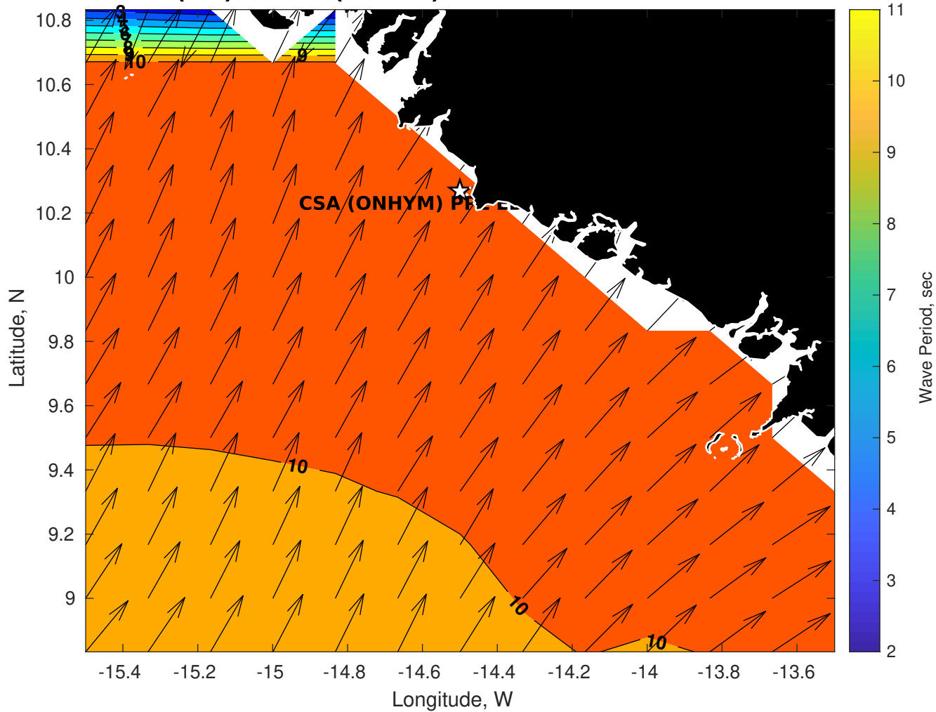
GFS Wave Period (sec) for CSA (ONHYM) PPL EBS - Guinea at 20-Dec-2025 09:00:00
