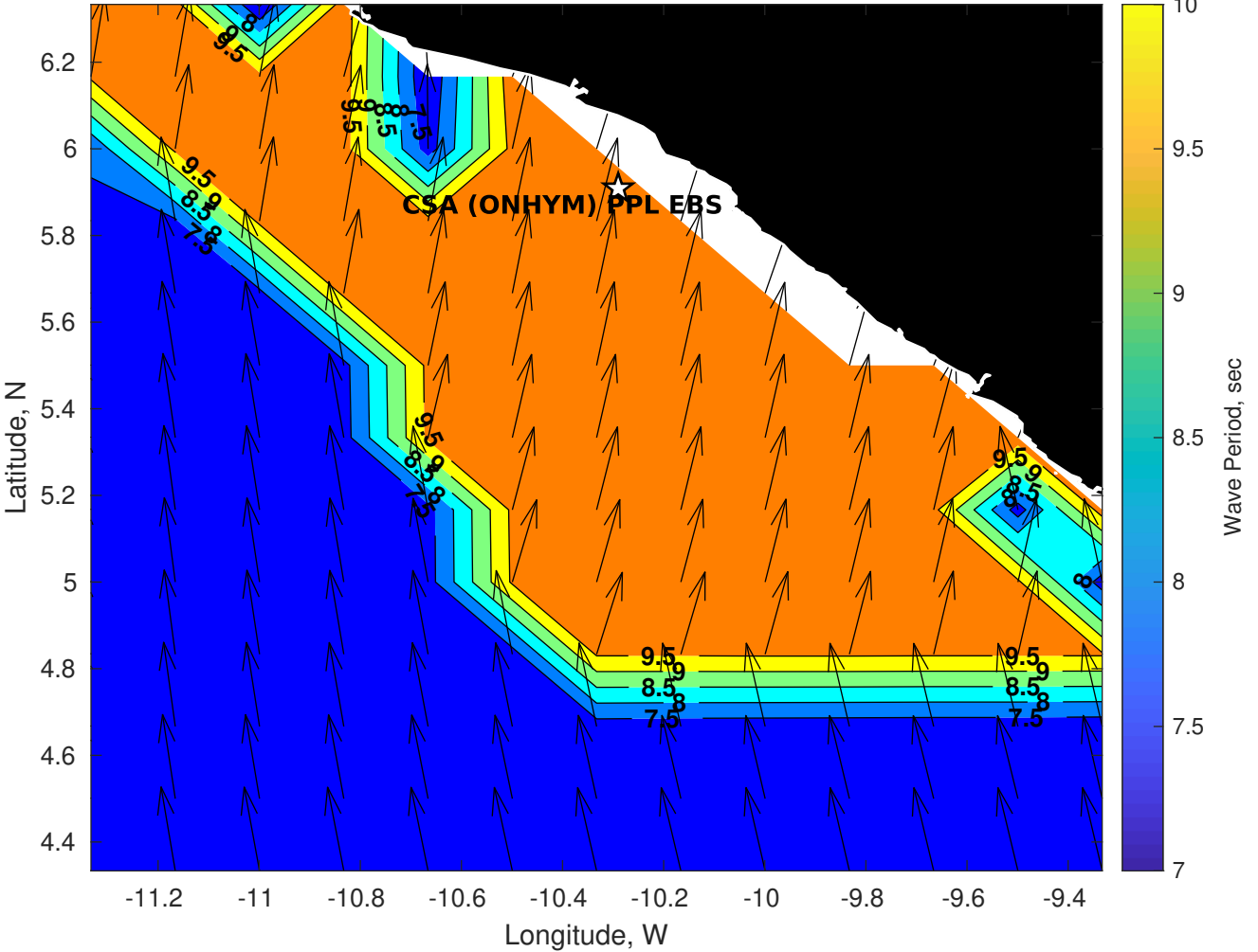
GFS Wave Period (sec) for CSA (ONHYM) PPL EBS - Liberia at 20-Dec-2025 09:00:00
