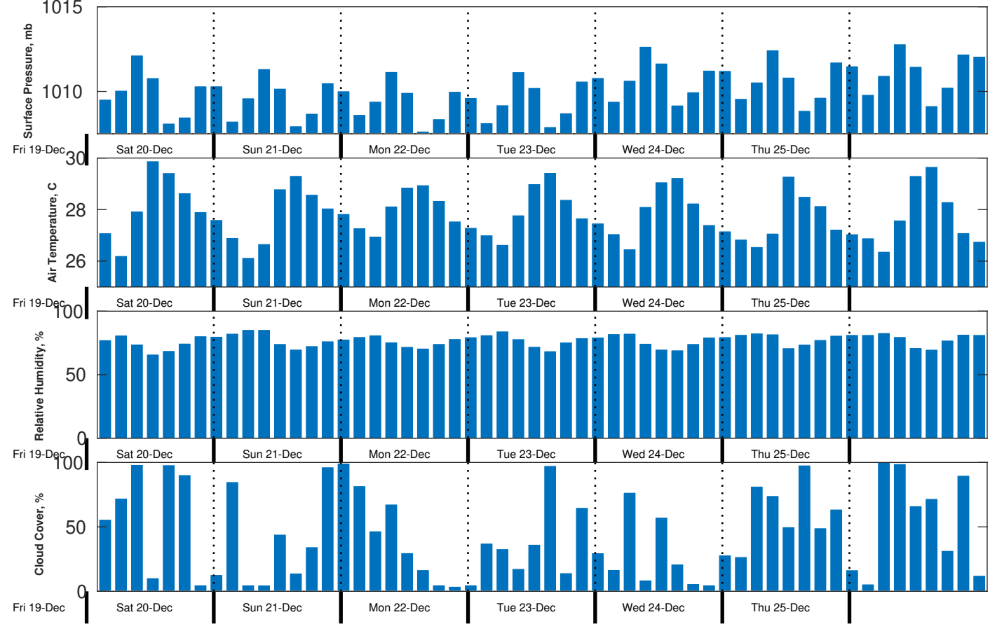
Met Forecast for CSA (ONHYM) PPL EBS - Liberia from 20-Dec-2025 00:00:00 to 27-Dec-2025 00:00:00
