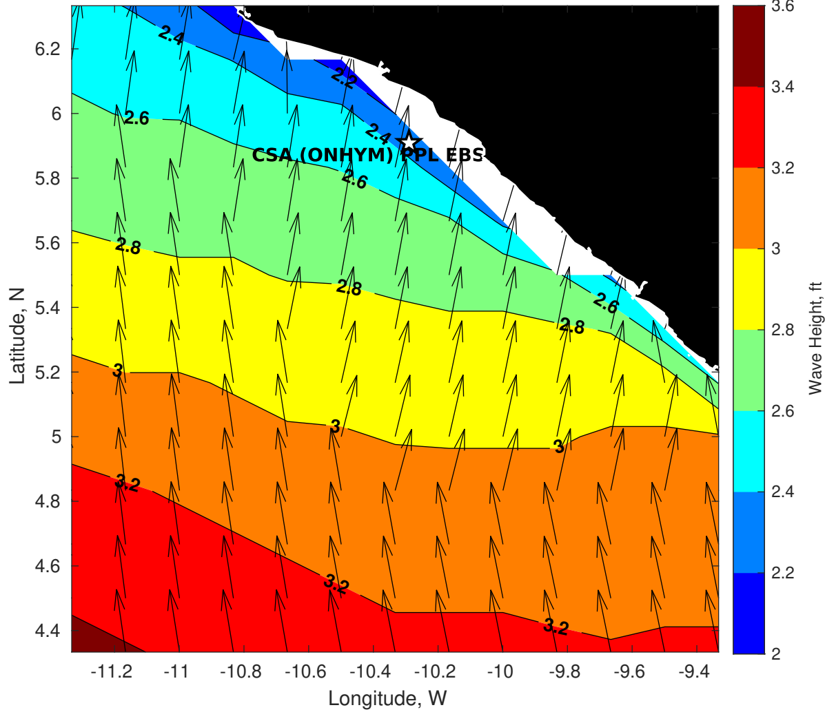
GFS Wave Height (ft) for CSA (ONHYM) PPL EBS - Liberia at 20-Dec-2025 09:00:00
