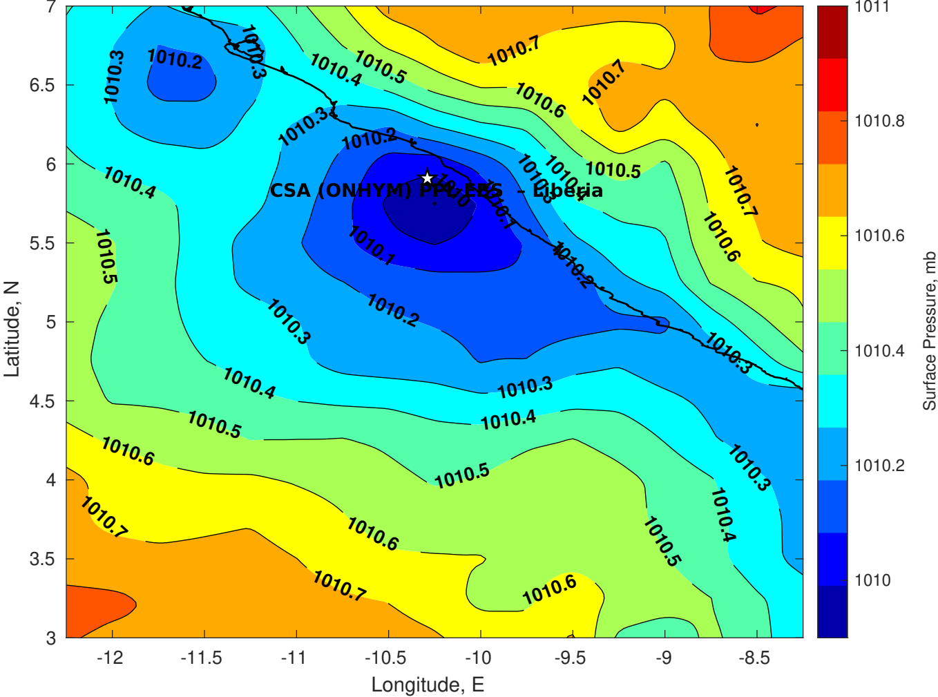
Surface Pressure (mb) for CSA (ONHYM) PPL EBS - Liberia at 22-Dec-2025 00:00:00
