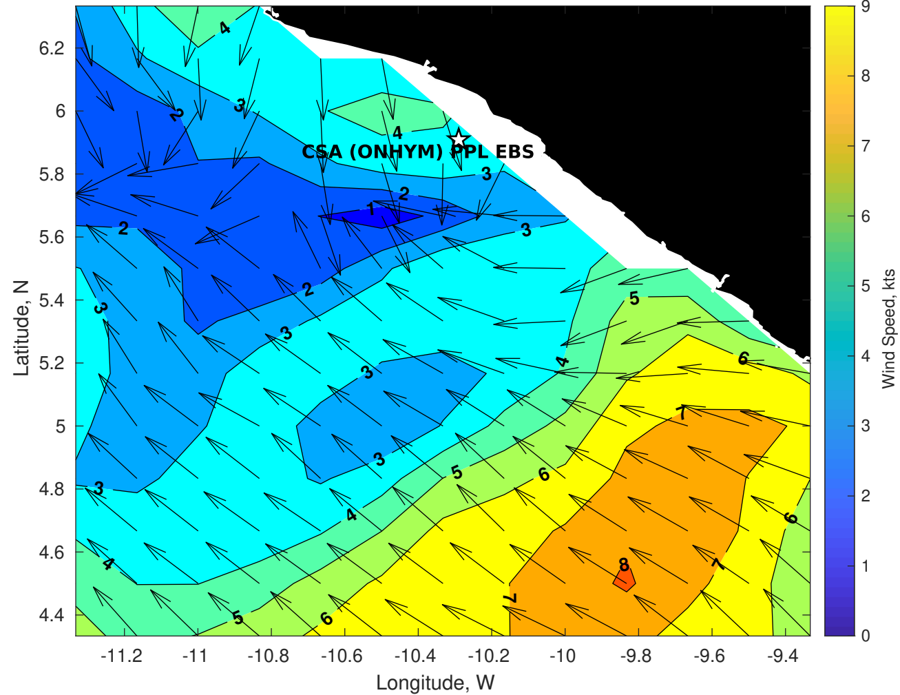
GFS Winds (kts) for CSA (ONHYM) PPL EBS - Liberia at 20-Dec-2025 09:00:00
