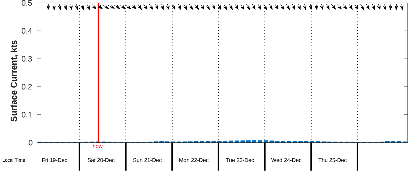
Surface Current Forecast for CSA (ONHYM) PPL EBS - Liberia from 19-Dec-2025 00:00:00 to 27-Dec-2025 00:00:00
