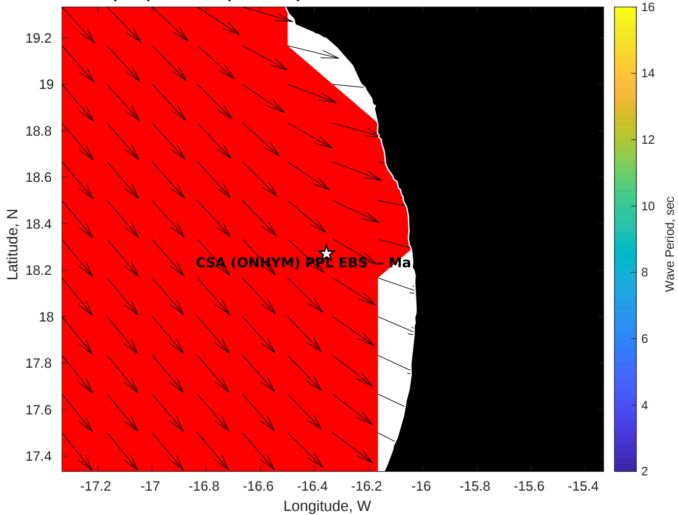
GFS Wave Period (sec) for CSA (ONHYM) PPL EBS - Mauritania at 20-Dec-2025 09:00:00
