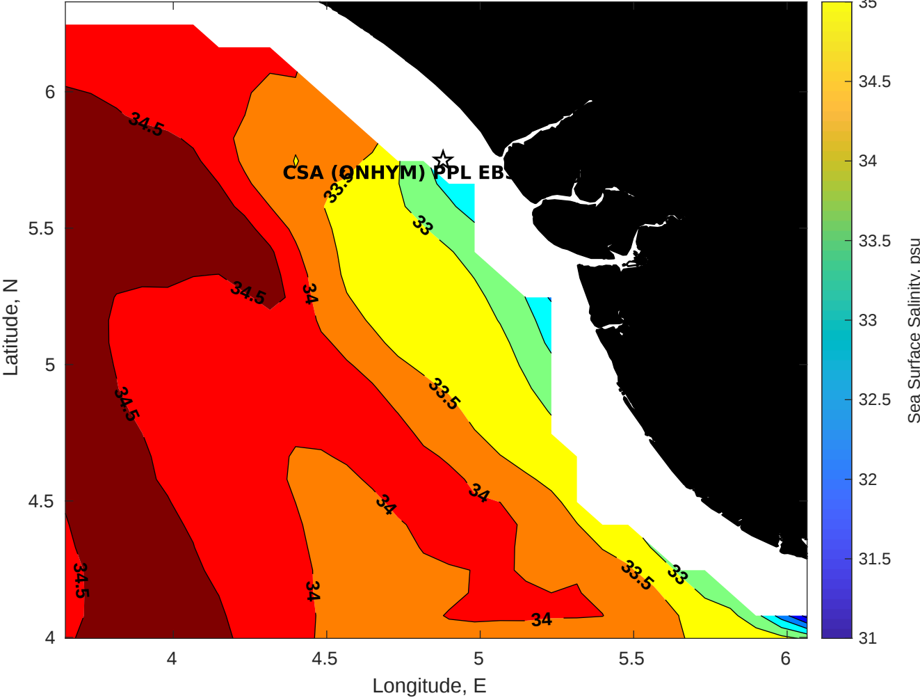
Surface Salinity for CSA (ONHYM) PPL EBS - Nigeria at 19-Dec-2025 00:00:00
