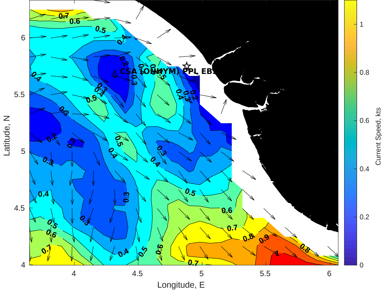
Surface Currents for CSA (ONHYM) PPL EBS - Nigeria at 19-Dec-2025 00:00:00
