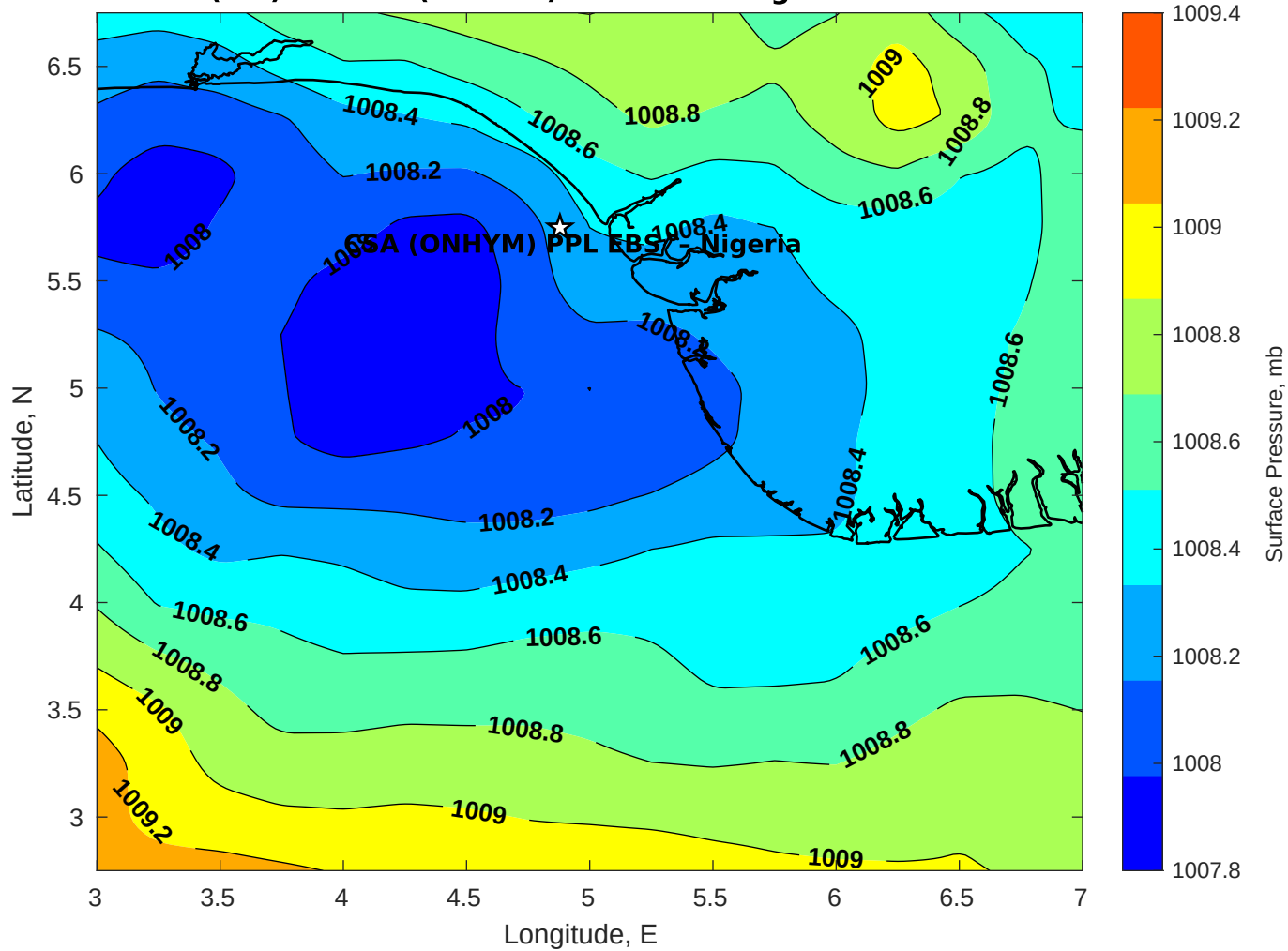
Surface Pressure (mb) for CSA (ONHYM) PPL EBS - Nigeria at 21-Dec-2025 00:00:00
