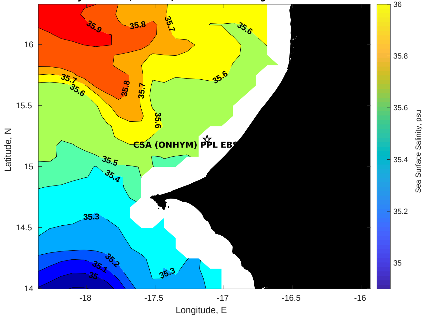
Surface Salinity for CSA (ONHYM) PPL EBS - Senegal at 19-Dec-2025 00:00:00
