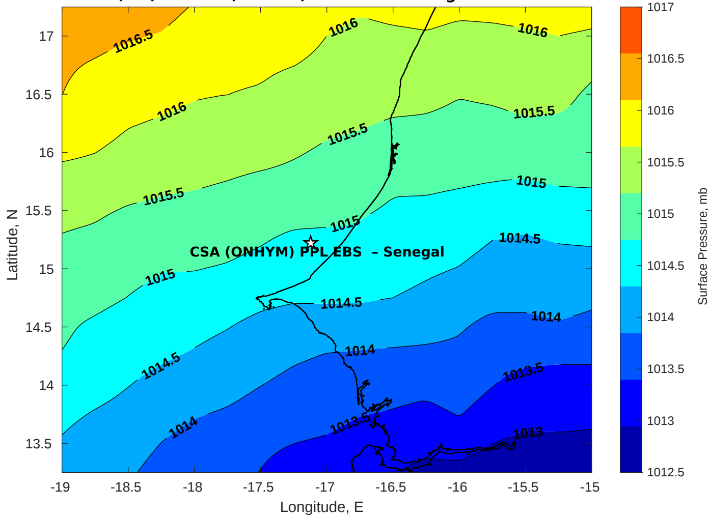
Surface Pressure (mb) for CSA (ONHYM) PPL EBS - Senegal at 20-Dec-2025 00:00:00
