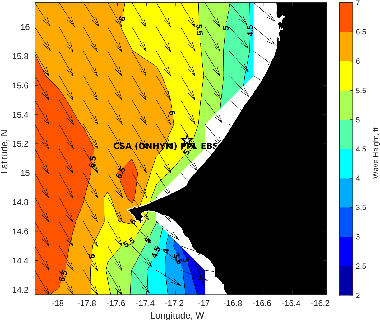
GFS Wave Height (ft) for CSA (ONHYM) PPL EBS - Senegal at 20-Dec-2025 09:00:00
